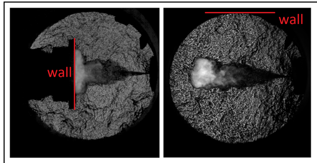
Figure 3. Schlieren imaging of the combustion. Left: jet impingement at a distance of 45 mm. Right: radiation test: the obstacle and heat flux sensor are placed away from the jet, and there is no impingement.
