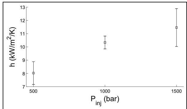
Figure 8. Convection coefficient variation with injection pressure.
