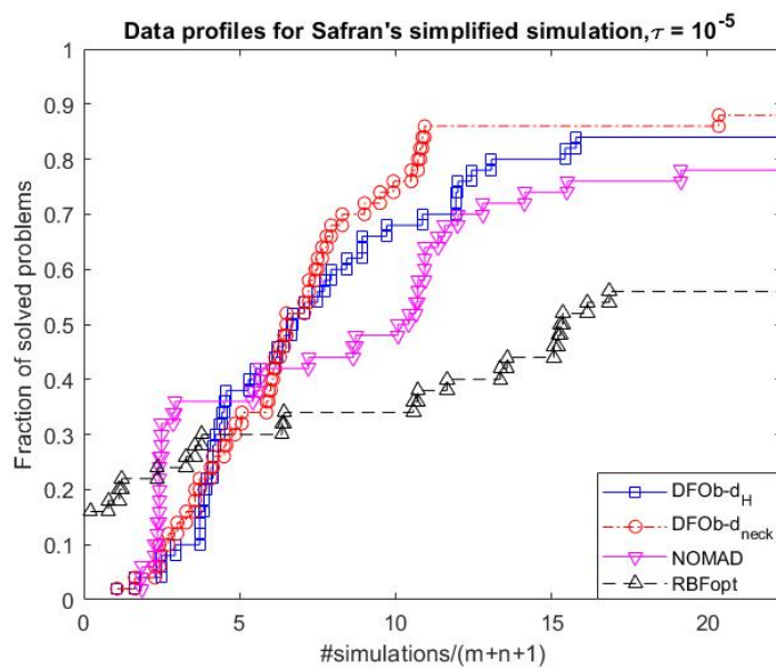
Fig. 6 Data profiles of the four solvers for the blade design application with 50 repetitions
