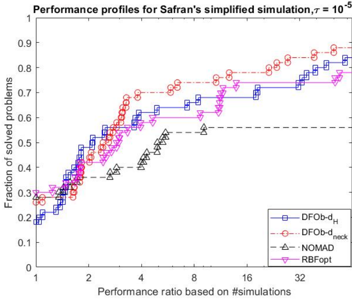
Fig. 5 Performance profiles of the four solvers for the blade design application with 50 repetitions
