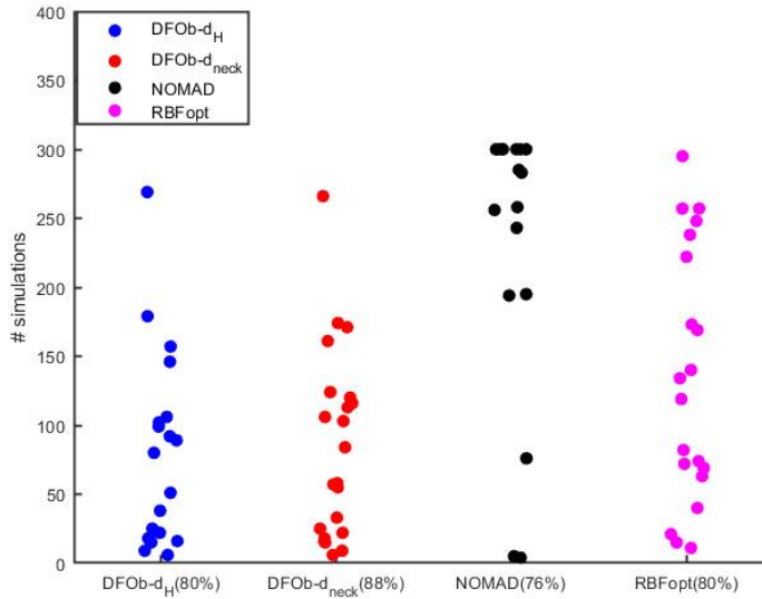
Fig. 4 Number of function evaluations to reach f^* up to \tau = 10^{-3} for each of the 25 analytical problems for the four solvers (successful runs only) together with percentage of success (in parentheses)
