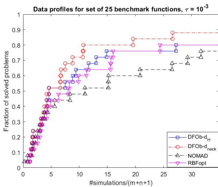
Fig. 3 Data profiles of the four solvers for the 25 analytical problems
