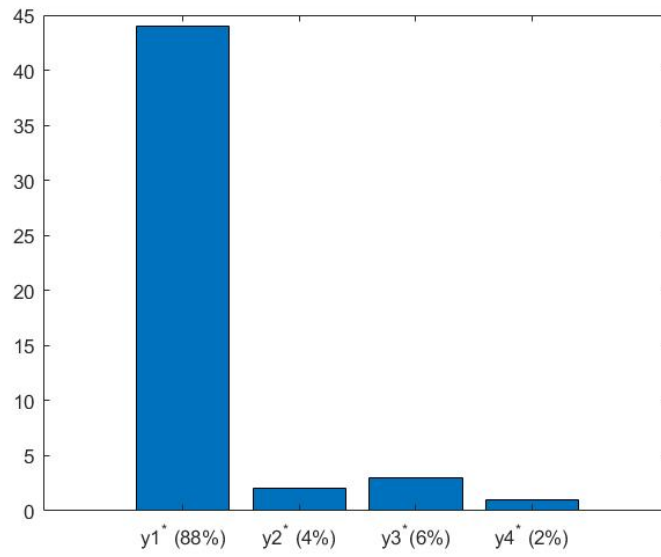
Fig. 8 Distribution of the binary component of the 50 solutions found by DFOb- d_{neck} for the blade design application.
