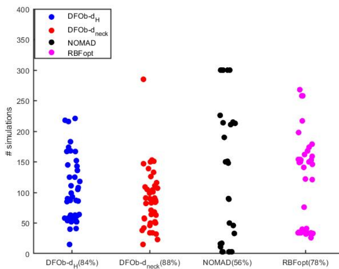
Fig. 7 Number of function evaluations to reach f^* up to \tau = 10^{-5} for each of the 50 runs of the blade design application for the four solvers (successful runs only) together with percentage of success (in parentheses)
