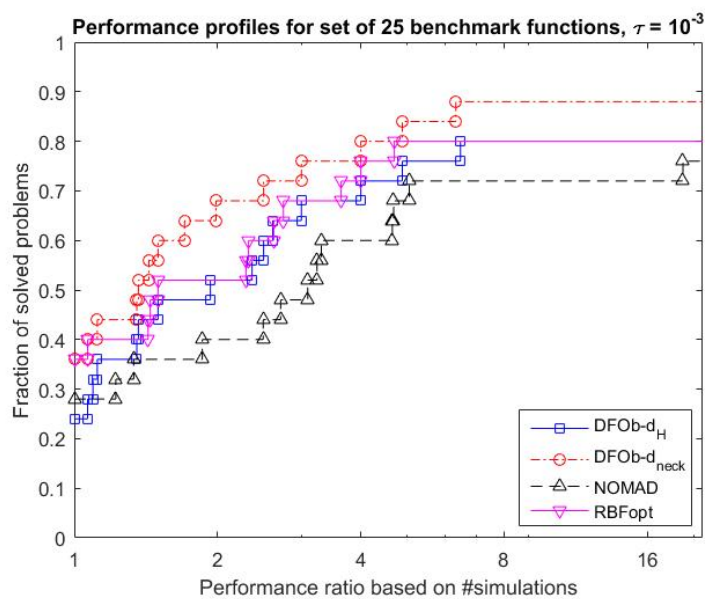
Fig. 2 Performance profiles of the four solvers for the 25 analytical problems
