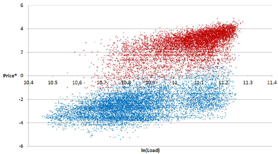
Figure 12. Price* vs. \ln(\text{Load}) for the two regimes (blue: regime 1, red: regime 2)
