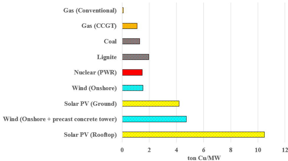
Fig. 4: Copper content of different energy means of production (kg/MW) considered in the model TIAM-IFPEN
