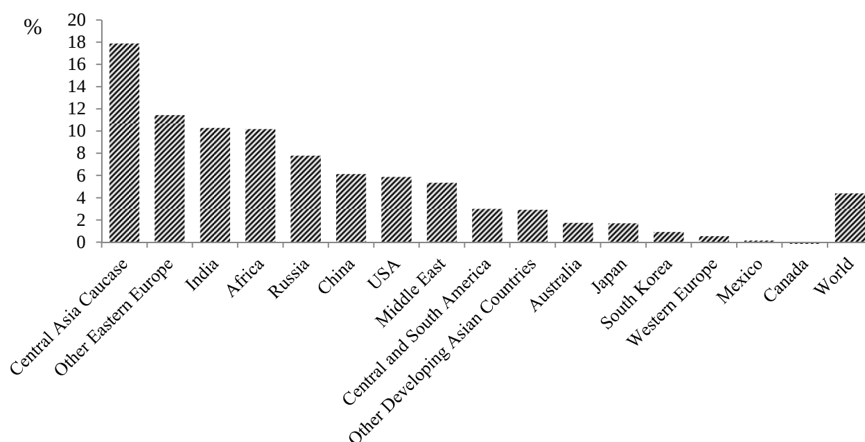
Fig. 10: Share of primary copper consumption avoided through a sustainable mobility scenario (in %), 2010-2055
