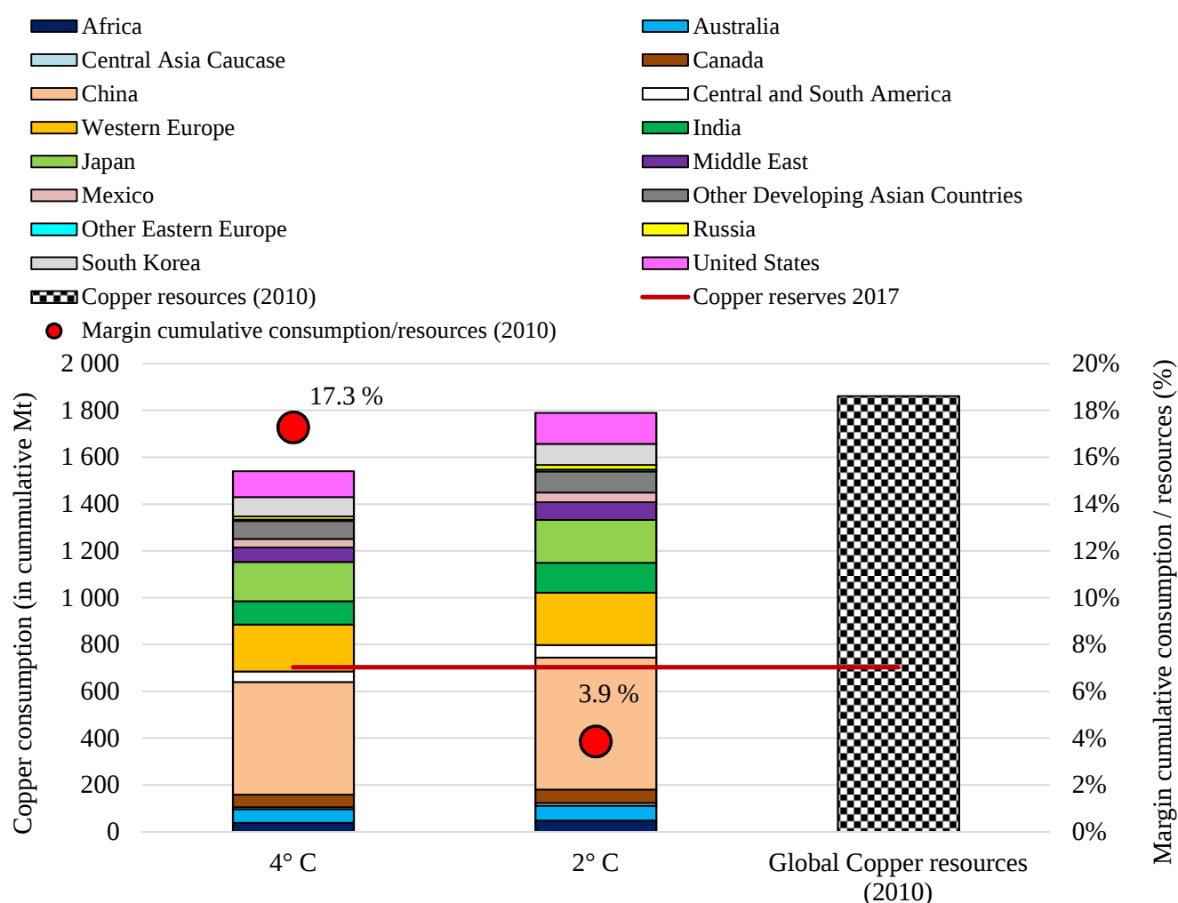
Fig. 6: Comparison between cumulative copper extraction from 2010 to 2055 under two climate scenarios and global copper resources in 2010
