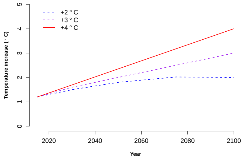
Fig. 9. Three prospective scenarios of temperature change (relatively to the pre-industrial era).
