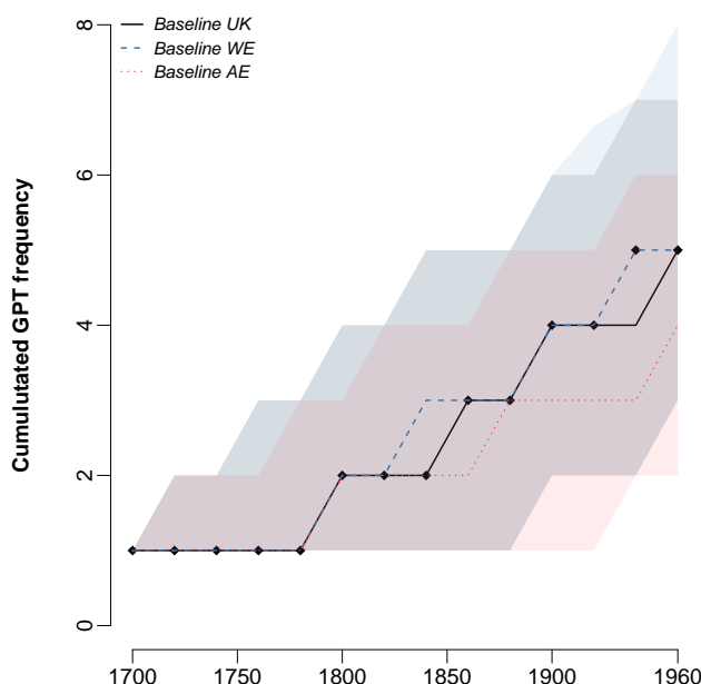
Fig. 9 GPT frequency in the baseline calibration (10,000 simulations) for Great Britain ( black ), Western Europe ( blue ) and Eastern Asia ( red ), 1700-1960 ( solid, dashed and dotted lines are medians, color shades are 90% probability intervals, diamonds are historical data ). Data source: Lipsey et al. (2005, p. 132)
