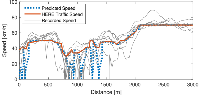
Fig. 2: Example of speed profile prediction via the modified IDM and the probabilistic stopping behavior model as compared to the HERE API traffic information and the real-world recorded speed profiles.
