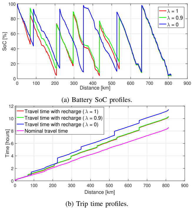
Fig. 4: Routing solution sensitivity to different values of \lambda .
