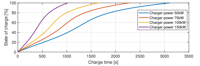
Fig. 1: Rapid charging time profile for a battery with a capacity of 30 kWh and different charger powers.
