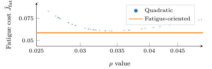
Fig. 4. Scatter plot of J_{fat}(\bar{x}_0, \mathbf{v}, \rho) in function of \rho and plot of the fatigue cost obtained using the fatigue-oriented optimization. For given \bar{x}_0 and \mathbf{v} , under a prediction horizon of 100 seconds and zoomed in the zone of interest.
