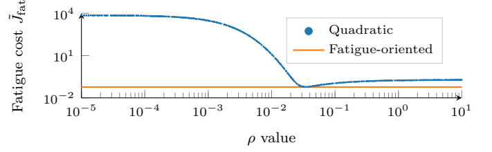
Fig. 3. Scatter plot of J_{fat}(\bar{x}_0, \mathbf{v}, \rho) in function of \rho and plot of the fatigue cost obtained with the fatigue-oriented optimization. For given \bar{x}_0 and \mathbf{v} , under a prediction horizon of 100 seconds and for 1000 values of \rho .
