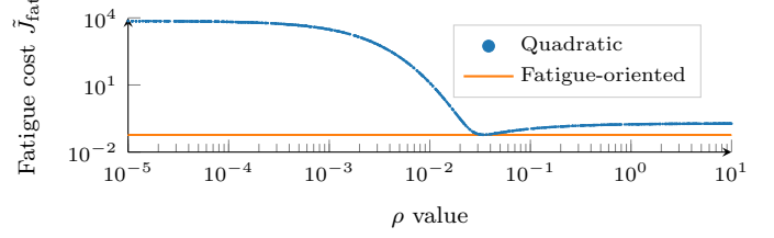
Fig. 3. Scatter plot of J_{fat}(\tilde{\mathbf{x}}_0, \mathbf{v}, \rho) in function of \rho and plot of the fatigue cost obtained with the fatigue-oriented optimization. For given \tilde{\mathbf{x}}_0 and \mathbf{v} , under a prediction horizon of 100 seconds and for 1000 values of \rho .
