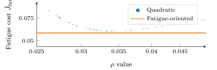
Fig. 4. Scatter plot of J_{fat}(\tilde{\mathbf{x}}_0, \mathbf{v}, \rho) in function of \rho and plot of the fatigue cost obtained using the fatigue-oriented optimization. For given \tilde{\mathbf{x}}_0 and \mathbf{v} , under a prediction horizon of 100 seconds and zoomed in the zone of interest.
