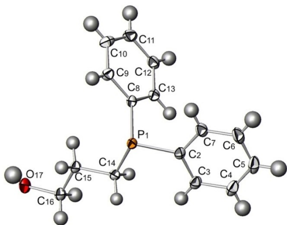
Figure 2. ORTEP view with full labelling scheme of 19·H. Thermal ellipsoids include 50% of the electron density. The H atom on O17 is disordered over two positions with 50/50 occupancy; only one is represented. Main distances (Å) and angles (°): P 1 –C 2 1.827(2), P 1 –C 8 1.834(2), P 1 –C 14 1.841(2), C 16 –O 17 1.420(2); C 2 –P 1 –C 8 99.8(1), C 2 –P 1 –C 14 102.2(1), C 8 –P 1 –C 14 100.7(1).
