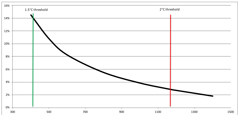
Fig. 3 Discounted global welfare cost in % of discounted GDP with respect to carbon budget in Gt CO 2
