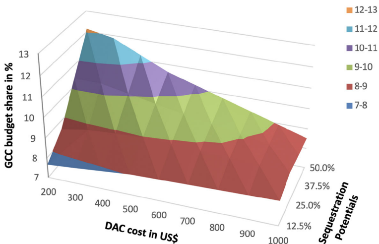
Fig. 5 Fair GCC budget share with respect the DAC cost and potential
