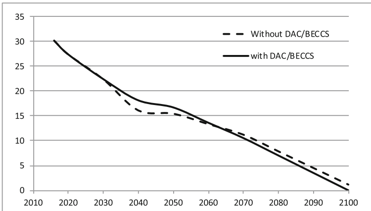
Fig. 1 Net emissions in Gt CO 2 with and without DAC/BECCS
