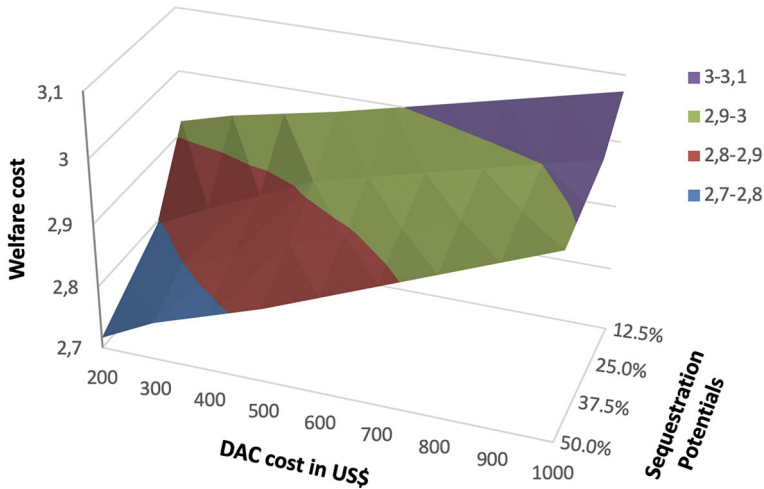
Fig. 4 Discounted global welfare cost in % of discounted GDP with respect the DAC cost and potential
