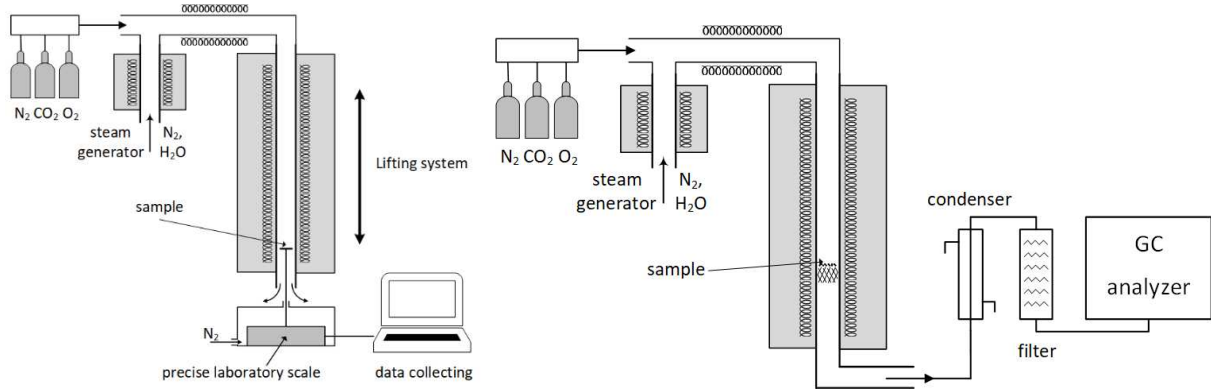
Fig. 2. The principle of petcoke gasification with the a) gravimetric and b) evolved gases methods
