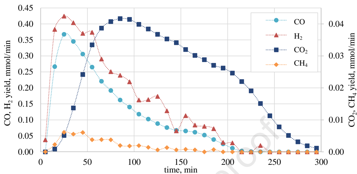
Fig. 3. Gas evolution profiles for petcoke gasification in 40 vol.% of steam in N 2 at 1000 □
