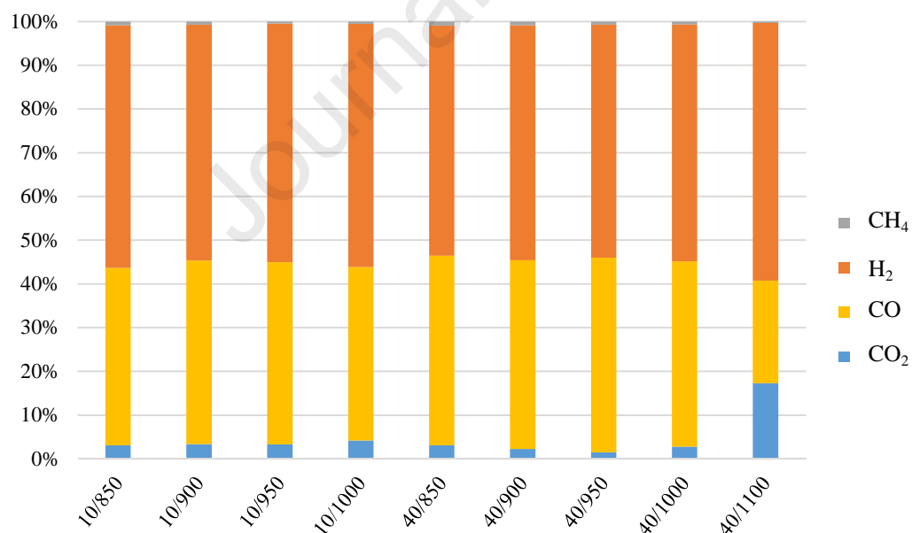
Fig. 4. Composition of the gaseous reaction products from petcoke steam gasification averaged for the conversion X = 0 to X = 0.5 (labels: steam concentration in vol.%/reaction temperature in □ )
