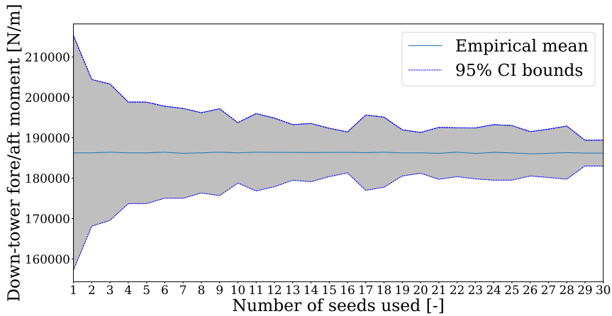
FIGURE 3 Convergence of the tower bottom fore-aft bending moment DEL as a function of the number of turbulent seeds used for its evaluation. 95% confidence interval around the estimated empirical mean is also represented (grey area). The wind turbulence intensity is set around 24 %, see [60].
