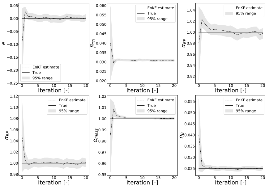
FIGURE 7 Iteration evolution of the a posteriori estimates of the input parameters. Results obtained by running EnKF presented in Section 2 with N = 100 members of the ensemble used for the estimation and considering pseudo-experimental numerical observations.
