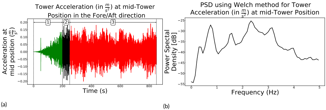
FIGURE 4 On the left side (a): simulated acceleration in \frac{m}{s^2} of the wind turbine tower in the fore-aft direction obtained at the accelerometer device located at mid-tower decomposed in a ramp time wind [1], an oversight period [2] and a dynamical period of interest [3]. On the right side (b): estimated PSD of the period of interest using Welch's method [68].
