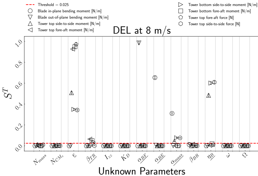
FIGURE 5 Estimation of total Sobol' indices (y-axis) with their 95% confidence interval corresponding to each of the 13 parameters (x-axis) for the different quantities of interest in fatigue. The dashed line corresponds to a threshold arbitrarily chosen to 2.5 \times 10^{-2} . Confidence intervals (CI) are obtained by taking into account the uncertainties due to both the metamodel and the Monte-Carlo estimation. The number of samples for the conditional Gaussian process, in order to quantify the uncertainty of the Kriging approximation, was set to 100. The uncertainty due to Monte-Carlo integration was computed with a bootstrap procedure with a sample size of 100.
