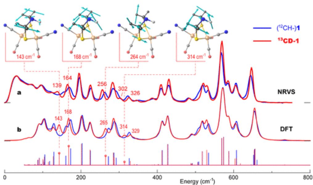
Figure 2. ^{57}\text{Fe} -PVDOS for the [2\text{Fe}]_n precursor isotopologues 1 (blue) vs ^{13}\text{CD-1} (red) from (a) NRVS experiments and (b) DFT calculations. Sticks correspond to individual DFT normal mode energies and intensities before lineshape convolution. For ^{13}\text{CD-1} , important band positions are labeled, and atomic motions in selected normal modes are shown.
