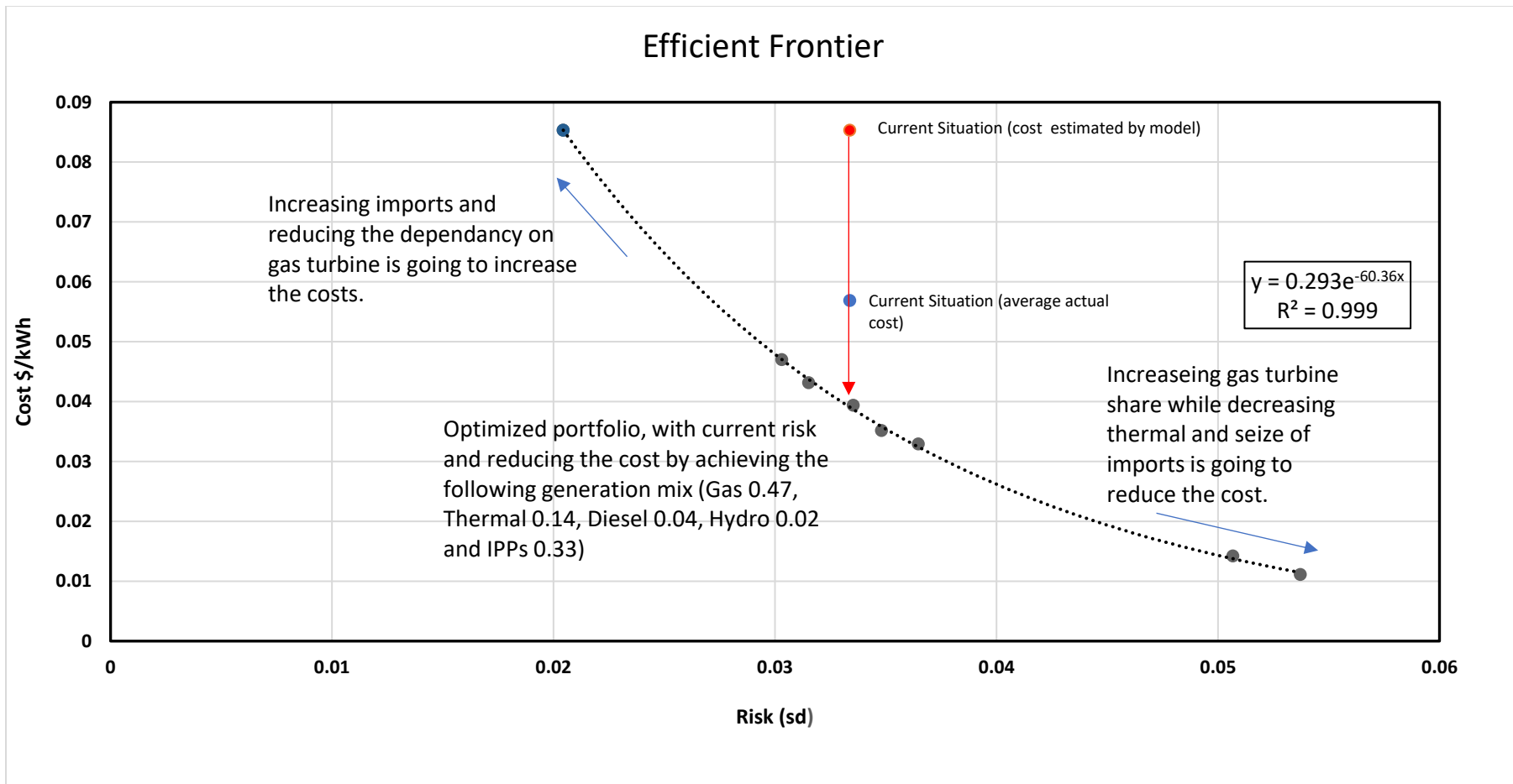
Figure 5: Efficient frontier and the optimization's results.
