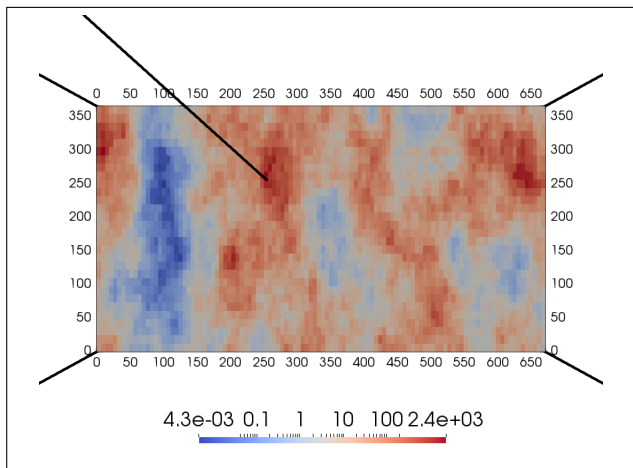
Fig. 8 Top view of the third illustration case permeability distribution with a log scale and the wells positions: 4 production wells are located at the corner of the model and 1 injection well is located at the center
