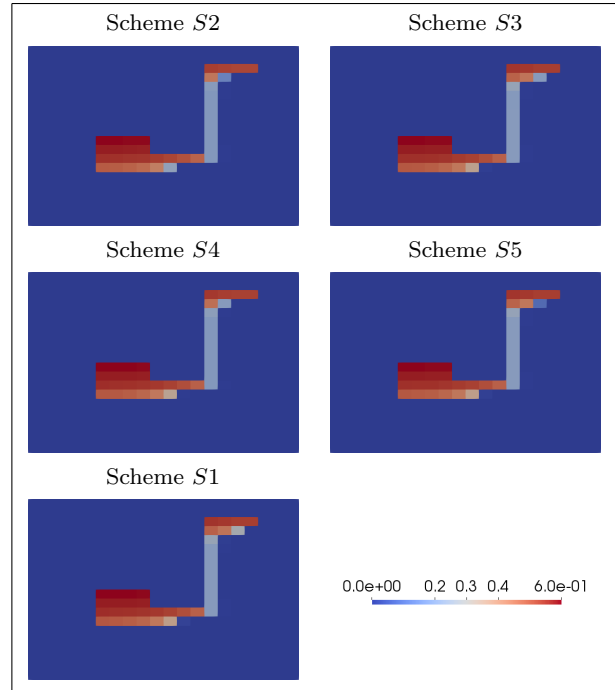
Fig. 6 Gas saturations at the end of the simulation for the second illustration case
