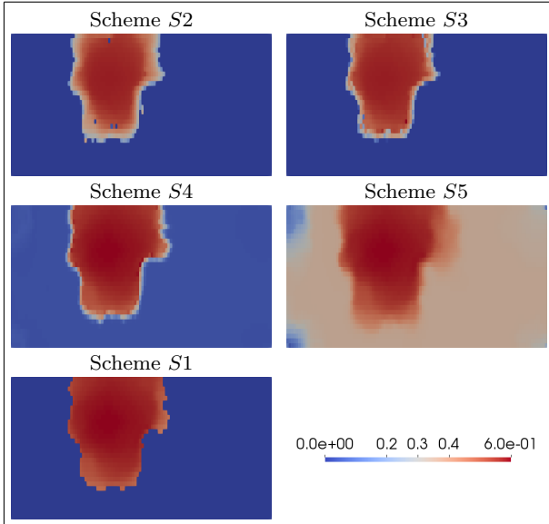
Fig. 9 Gas saturations at the end of the simulation for the SPE10 test case
