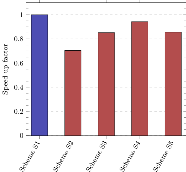
Fig. 4 Speed up factor for the 5 schemes compared to scheme S1 : a value below 1 means a longer run, a value higher than 1 means a speed up
