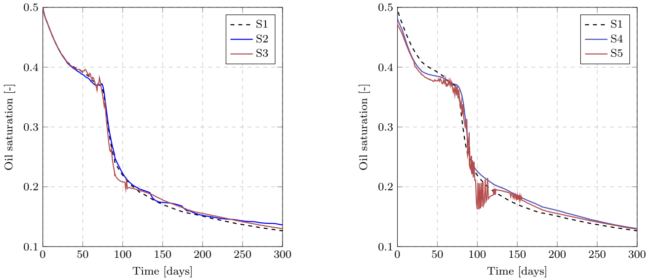
Fig. 3 Oil saturation as a function of time in the production well. In dashed black, for scheme S1 ; in blue, schemes using type I interpolation (schemes S2 and S4 ); in red, schemes using type II interpolation (schemes S3 and S5 ). In all the situations, the schemes using type I interpolation give smoother results than the schemes using type II interpolation
