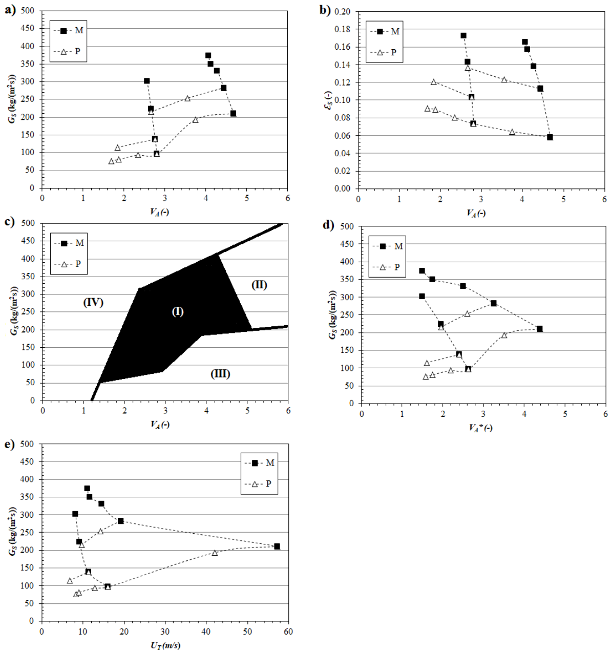
Fig. 5. Experimental data for injection of sawdust S_2 : a) G_S versus V_A , b) \epsilon_S versus V_A , c) operation map, d) G_S versus V_A^* , and e) G_S versus U_T .
