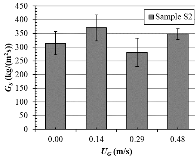
Fig. 10. Solids flux ( G_S ) for the injection of S_2 to fixed and fluidized beds under different unit gas velocities ( U_G ).
