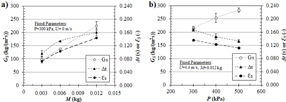
Fig. 3. Experimental solids flux ( G_S ), mean solids fraction ( \varepsilon_s ), and injection time ( \Delta t ) for sawdust S_2 as a function of operation parameters a) M , and b) P .
