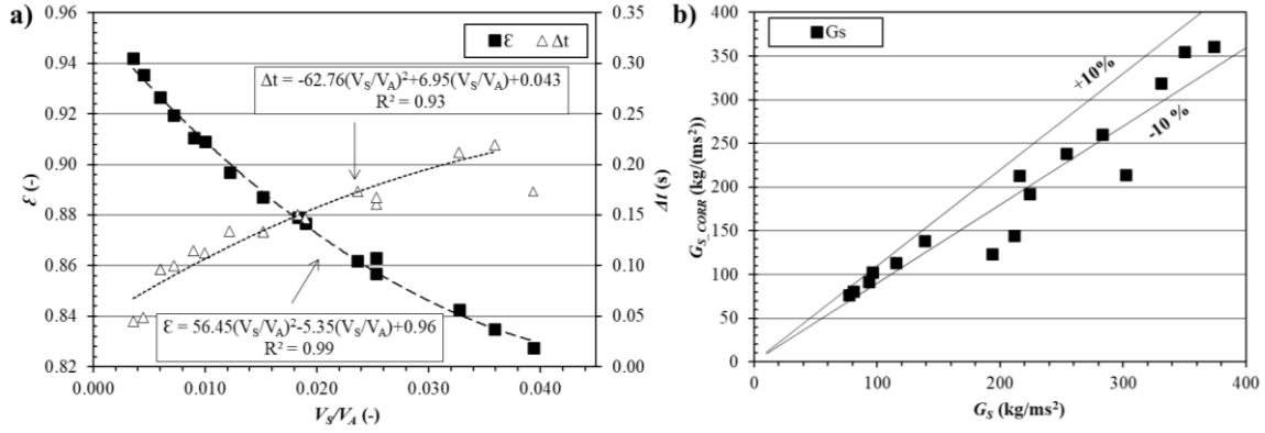
Fig. 7. Results for a) \varepsilon versus V_S/V_A , and b) fitting response for G_S .
