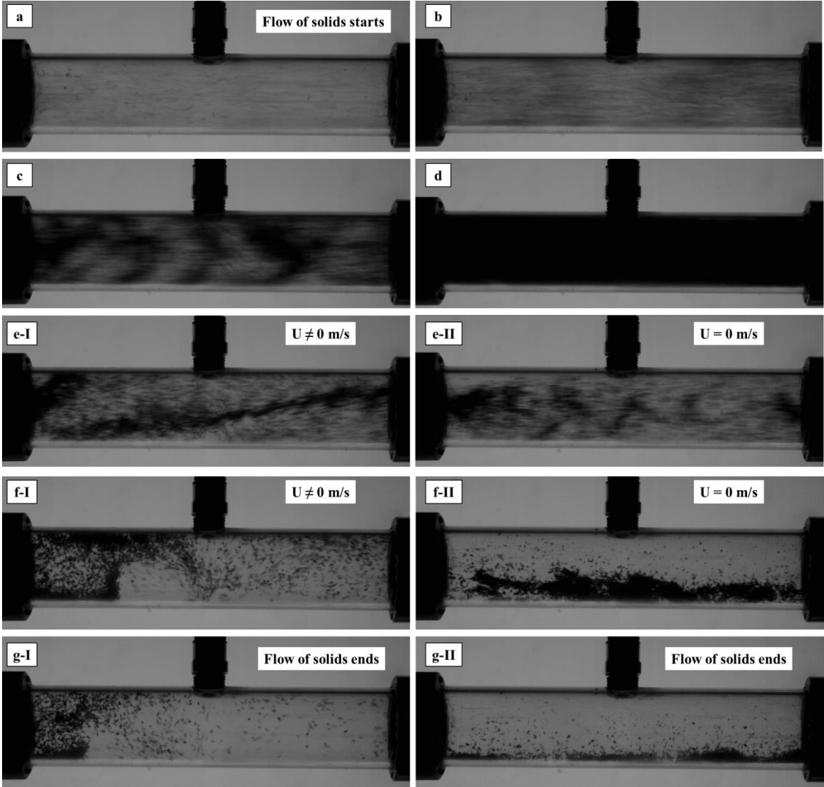
Fig. 2. Sequences of gas-solid hydrodynamics at the injection line for U \neq 0 m/s (Fig. 2a to 2g-I) and U=0 m/s (Fig. 2a to 2g-II).
