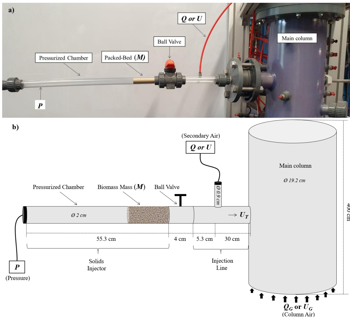
Fig. 1. Powders' injection system and principal variables investigated: P , M , Q or U , and Q_G or U_G . a) experimental unit and b) unit scheme with dimensions in cm as indicated.
