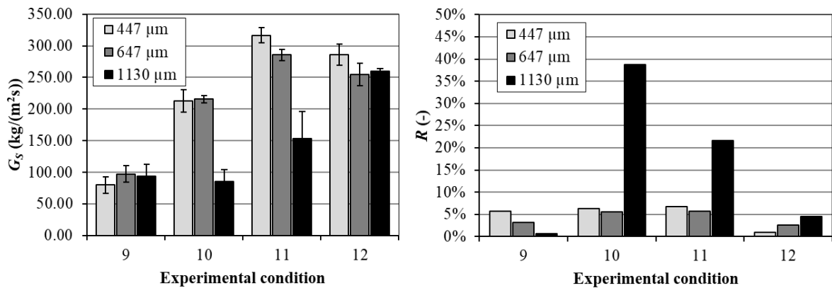
Fig. 8. Results of a) solids flux ( G_S ) and b) residual mass of solids ( R ) for the injection of three sawdust samples under different experimental conditions.
