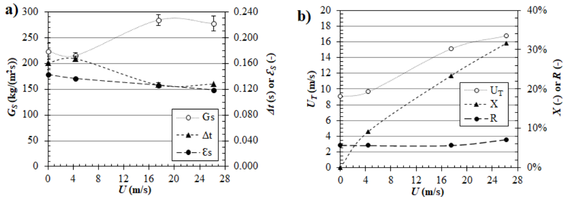
Fig. 6. Effect of U on a) G_S , \varepsilon_s , and \Delta t , and on b) U_T , R and X .
