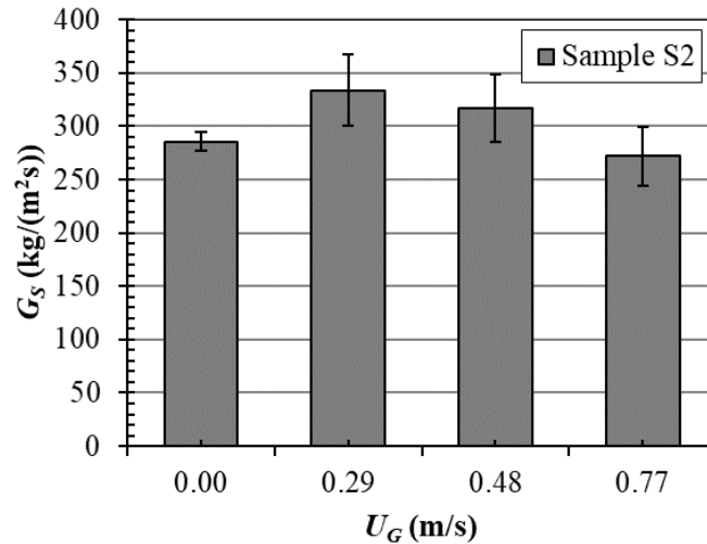
Fig. 9. Solids flux ( G_S ) for the injection of S_2 under different gas velocities in the unit ( U_G ).
