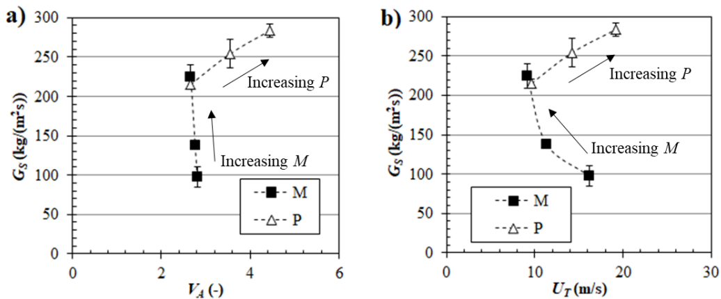
Fig. 4. Experimental solids flux ( G_S ) as a function of a) V_A , and b) U_T .
