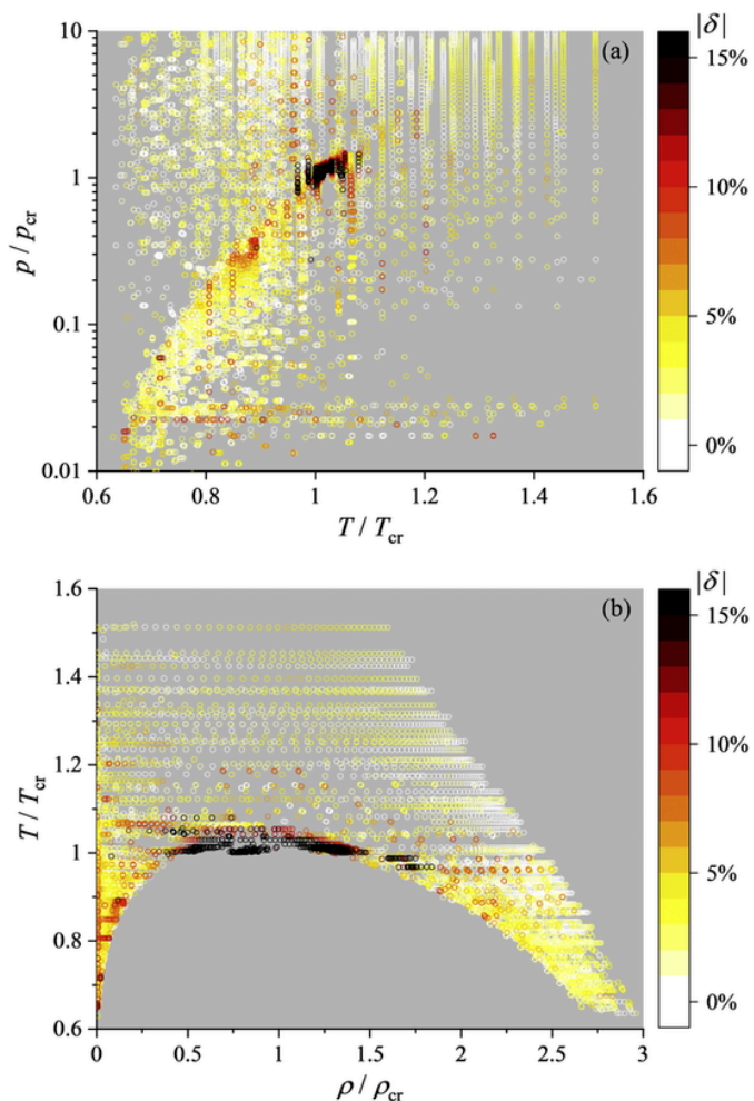
Fig. 6. Relative deviation in the reduced ranges of temperature, pressure, and density relative to their values at the critical point.
