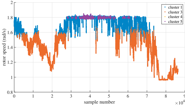
Fig. 2. Rotor speed time-series corresponding to Fig. 5. The points are color coded according to the cluster used for the estimation of the wind speed at the corresponding time.
