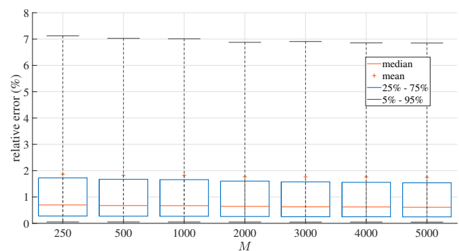
Fig. 9. Relative error for different values of M . The remaining parameters are C = 5 , r = 20 , and N = 10^4 . We use only the nearest cluster estimate.
