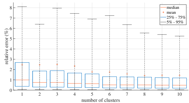
Fig. 8. Relative error for different choices of number of clusters. In this case r = 20 , N = 10^4 , M = 3000 , and we only use the nearest cluster estimate.
