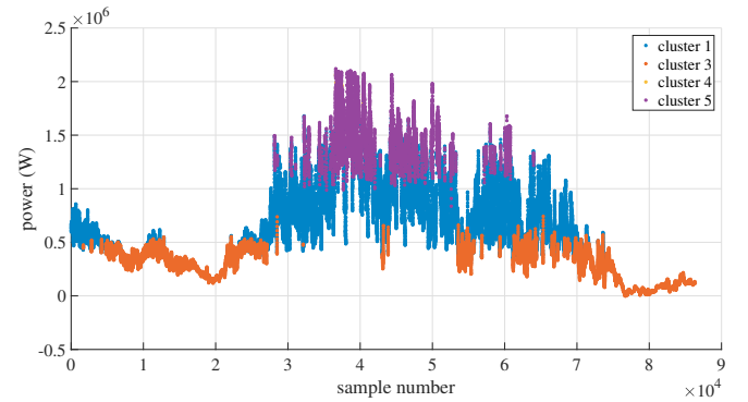
Fig. 4. Produced power time-series corresponding to Fig. 5. The points are color coded according to the cluster used for the estimation of the wind speed at the corresponding time.
