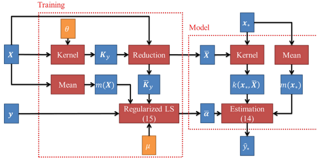
Fig. 1. Schematic of the algorithm for one cluster.
