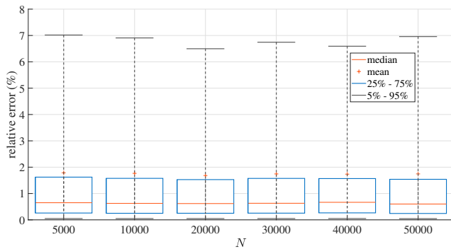
Fig. 10. Relative error for different values of N . The remaining parameters are C = 5 , r = 20 , and M = 3000 . We use only the nearest cluster estimate.
