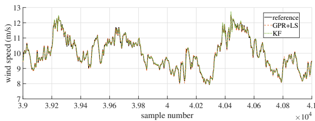
Fig. 6. Zoomed-in view of Fig. 5, with comparison to a Kalman Filter (KF) approach.
