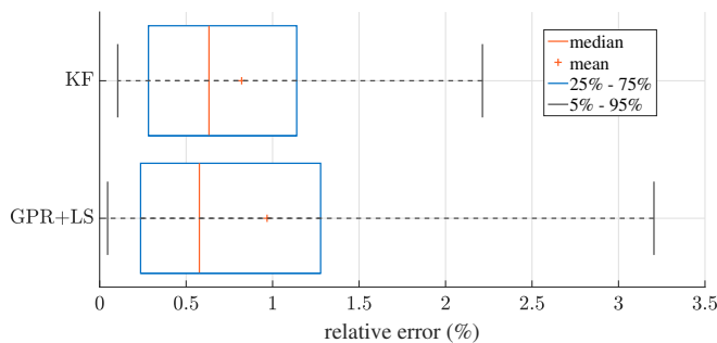
Fig. 7. Boxplots of the estimation error for the day shown in Figs. 5 and 6.
