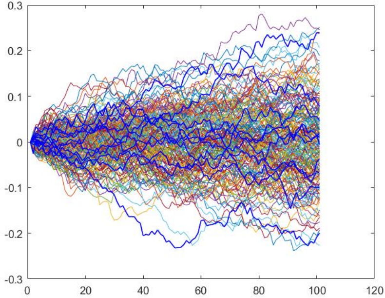
Figure 6: 200 realizations of a Brownian motion: the thick blue curves are the 10 curves selected by the first iterations of the Adapted-Greedy algorithm.
