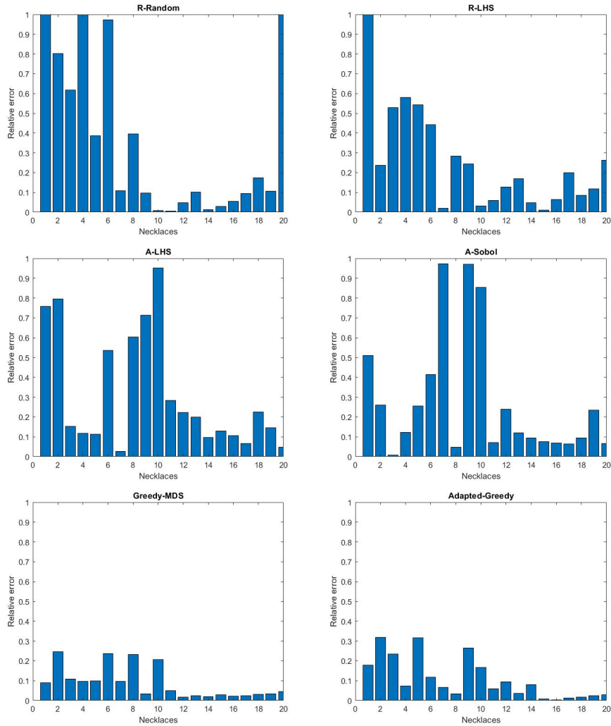
Figure 3: Distributions of estimation errors for each of the 20 necklaces of the Branin-nl function obtained with 6 methods: random sampling and standard LHS with rounded values for the binary variables, 2 projected methods based on Sobol sequence and projected LHS, the Greedy-MDS and Adapted-Greedy methods, for n_{DoE} = 100 .
