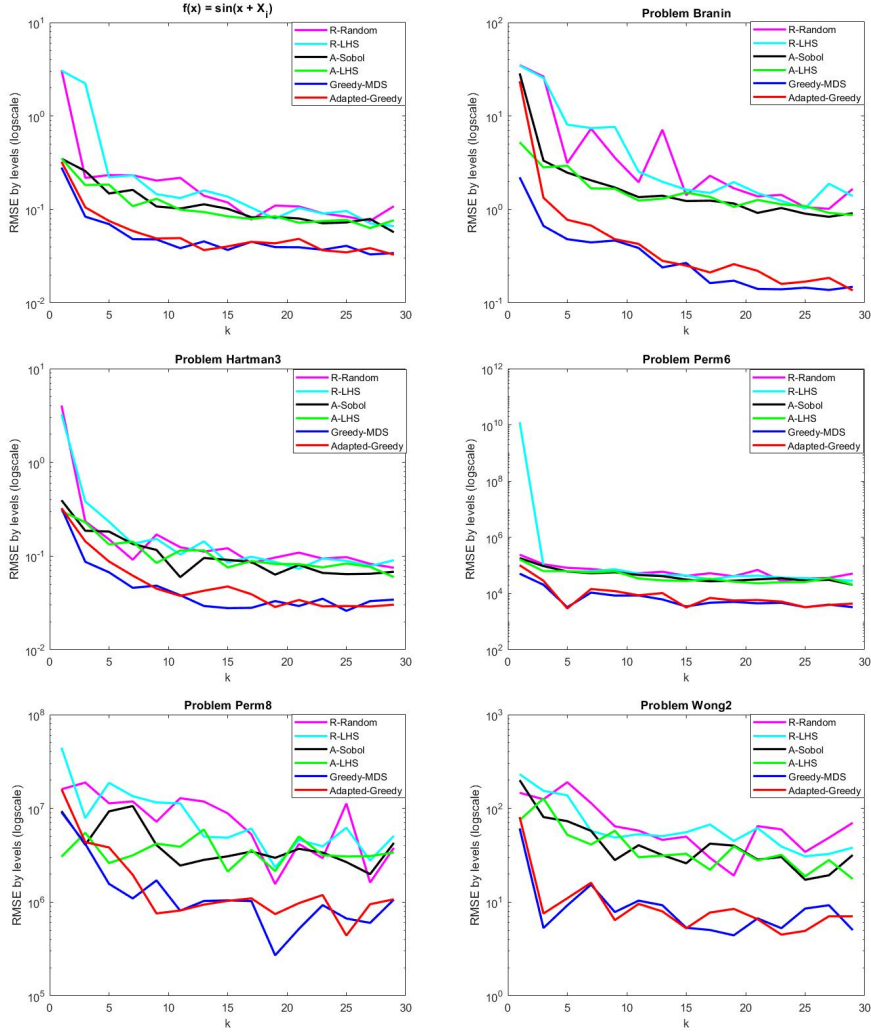
Figure 2: Median RMSE (in logscale) of the estimation of benchmark function expectation obtained with 5 repetitions of the 6 methods: a random sampling and a standard LHS with rounded values for binary variables, 2 projected methods based on Sobol sequence and projected LHS, the Greedy-MDS and Adapted-Greedy methods, for n_{DoE} = kn_{neck} .
