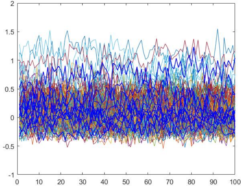
Figure 7: 200 realizations of a Max-stable process. The thick blue curves are the 10 curves selected by the first iterations of the Adapted-Greedy algorithm.
