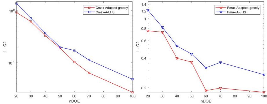
Figure 1: Accuracy of the surrogate models of the maximal torque (left) and the maximal power (right) built with designs of experiments obtained by the projected LHS method (in blue) and by the Adapted-Greedy algorithm (in red) with respect to the size of the designs.
