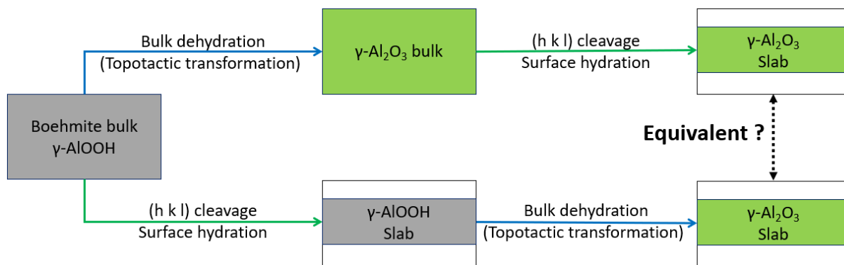
Scheme 1: Two ways of forming \gamma -Al 2 O 3 surfaces involving the topotactic transformation from boehmite. Top path: topotactic transformation applied to the bulk, bottom path: topotactic transformation applied to the slabs. The topotactic transformation method is taken from Ref. [30]
