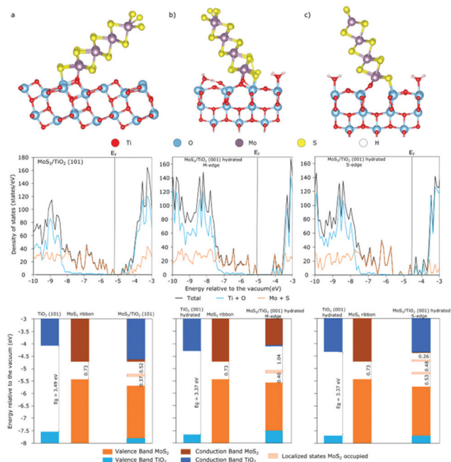
Fig. 6 Molecular structures of MoS 2 nanoribbons chemically adsorbed on the two TiO 2 surfaces, DOS of the interfaces and evolution of the bands positions before and after junction for (a) TiO 2 (101) (interaction with M-edge) and (c) TiO 2 (001) (interaction with S-edge).
