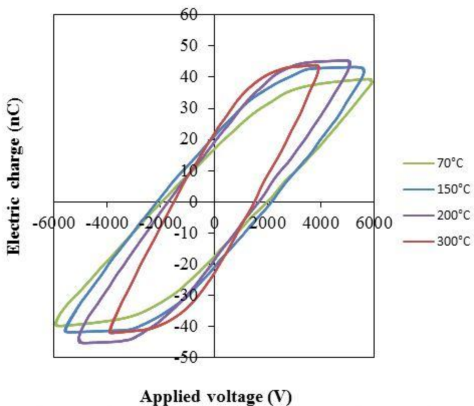
Figure SI-1: Lissajous figure for P=5W at 70, 150, 200 and 300°C during plasma treatment
