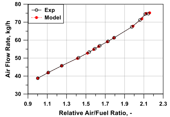
Figure 6. Experimental/numerical air flow rate comparison against the relative air/fuel ratio.
