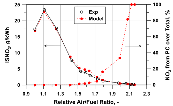
Figure 16. Experimental/numerical ISNO 2 comparison against the relative air/fuel ratio.
