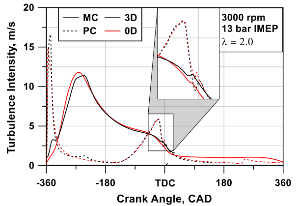
Figure 5. 1D/3D comparison of turbulence intensity in PC and MC.
