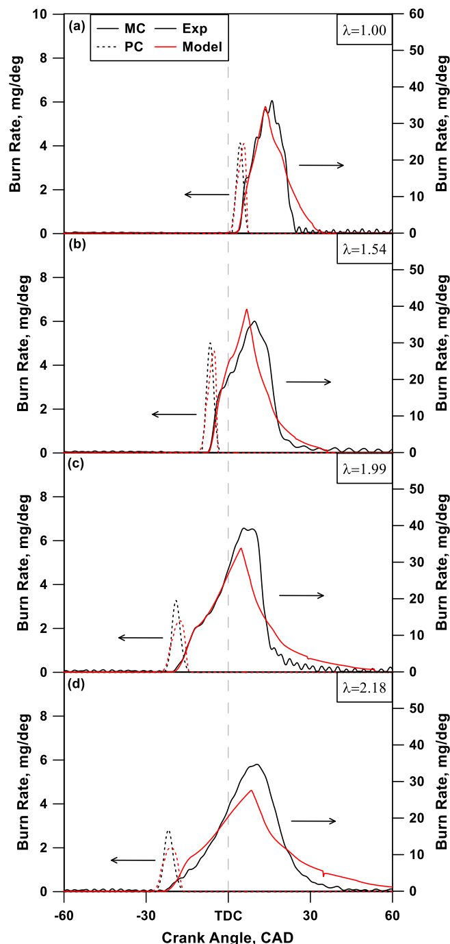
Figure 15. Experimental/numerical comparison of MC and PC burn rates at (a) \lambda=1.00 , (b) \lambda=1.54 , (c) \lambda=1.99 , (d) \lambda=2.18 .
