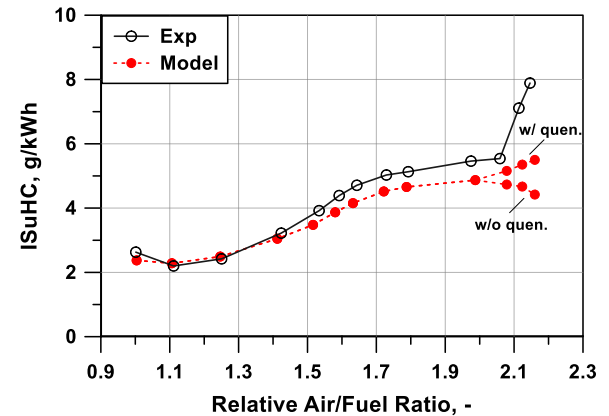
Figure 17. Experimental/numerical ISuHC comparison against the relative air/fuel ratio.
