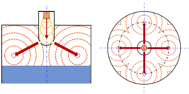
Figure 2. Flame front schematizations in PC and MC.
