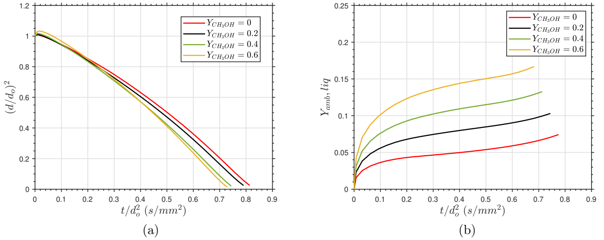
Figure 4.3: (a) Temporal evolution of the dimensionless squared droplet diameter (d/d_0)^2 and (b) mean mass fraction of dissolved ambient gases (methanol + nitrogen) in the liquid phase ( Y_{amb,liq} ) at ( P_{amb} = 106 bar, T_{amb} = 1200 K) for different methanol ambient concentrations ( Y_{CH_3OH} ).
