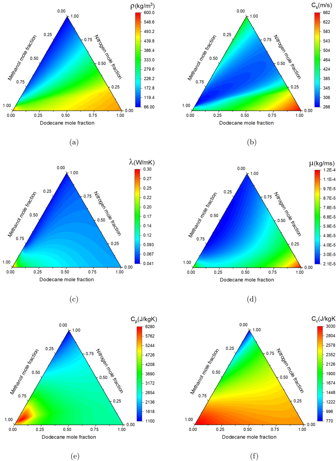
Figure A.2: Contour plots of the ternary (n-dodecane/nitrogen/methanol) mixture thermodynamic and transport properties at ( P = 106 bar, T = 500 K). (a) density (b) sound speed (c) thermal conductivity (d) dynamic viscosity (e) isobaric heat capacity (f) isochoric heat capacity.
