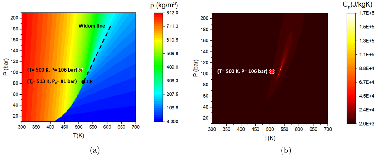
Figure A.3: Pressure-temperature diagram of pure methanol ( CH_3OH ). (a) Density contours mapped with the widom line and the critical point (CP) (b) isobaric heat capacity contours. The red cross indicates that ( P = 106 bar and T = 500 K) is at the vicinity of the widom line, where the isobaric heat capacity reaches a peak value.
