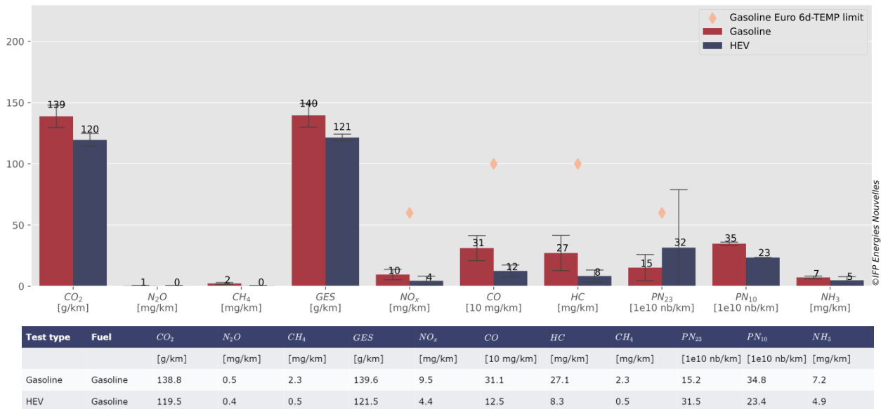
Figure 18 : Comparison of the average emissions of the gasoline and hybrid vehicle selected on the experimental protocol.
