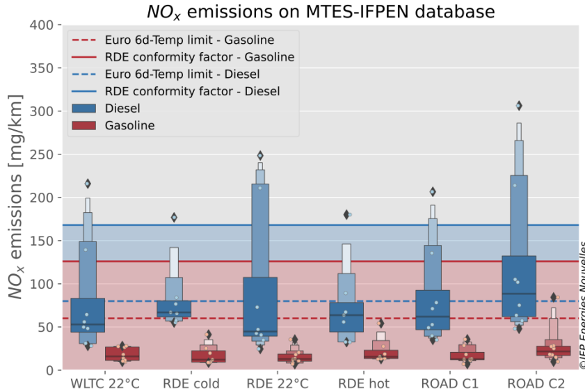
Figure 15 : Comparison of NOx emissions from gasoline and diesel vehicles for each type of test performed
