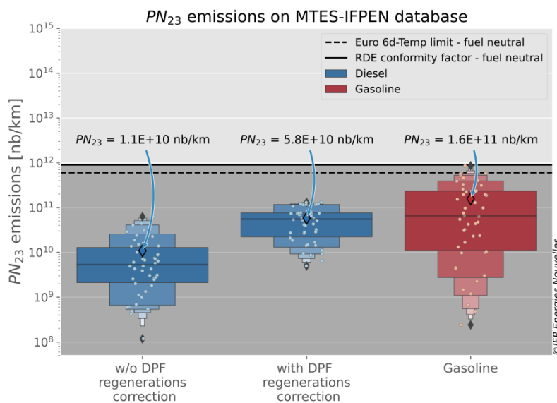
Figure 11 : Comparison of number of particulate emissions over 23 nm from gasoline and diesel vehicles over the full scope of the study
