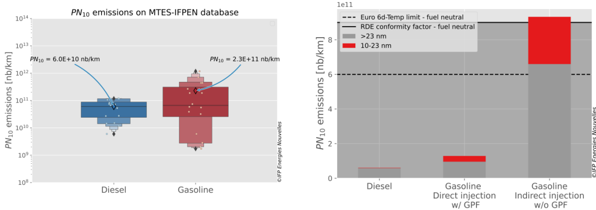
Figure 14 : Comparison of number of particle emissions of more than 10nm from gasoline and diesel vehicles on the scope of non-climatic chassis dynamometer tests
