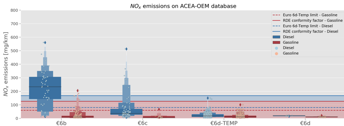
Figure 4 - Manufacturer's NO x emissions data on RDE. Sources: ACEA and JAMA
