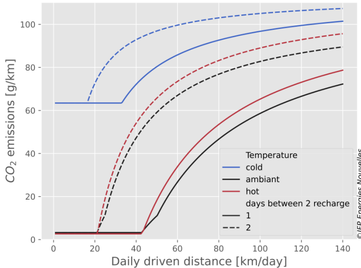
Figure 25 : Impact of the test temperature on CO 2 emissions according to use for PHEV gasoline SUV : comparison of RDE tests on cold (-2 °c), nominal (22 °c) and hot ( 35 °c). Road tests are excluded from the considered perimeter to isolate the temperature effect on identical routes.
