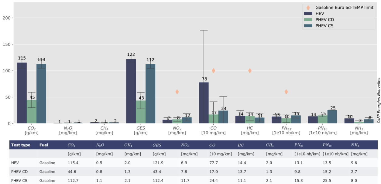
Figure 19 : Comparison of the average emissions of the non-rechargeable hybrid (HEV) and plug-in hybrid vehicle selected on the experimental protocol.
