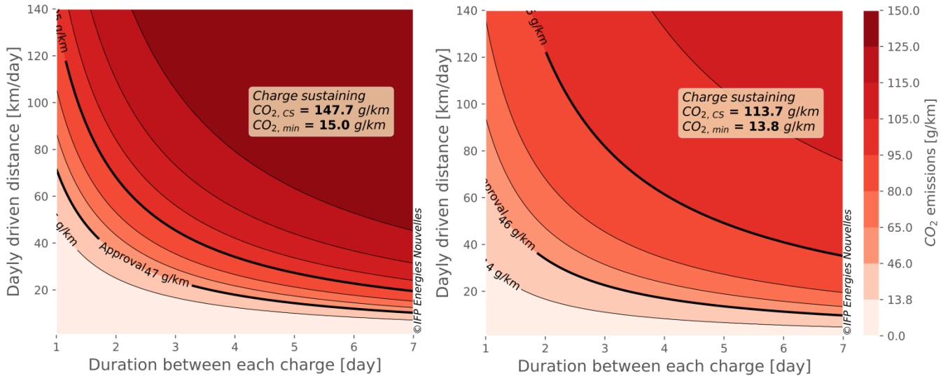
Figure 23 - CO2 emissions from PHEV gasoline (left) and diesel (right) vehicles, depending on the frequency of recharging and the length of daily trips. The approved CO2 score is also shown (Approval). Tests on a climatic chassis dynamometer are excluded from the considered scope.
