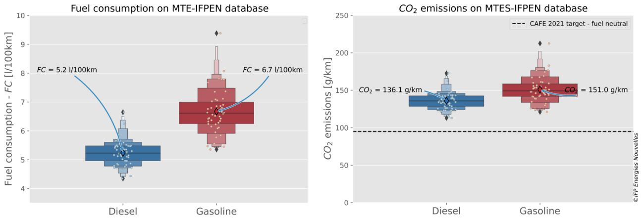
Figure 7 : Comparison of CO 2 emissions and fuel consumption of gasoline and diesel vehicles over the full scope of the study
