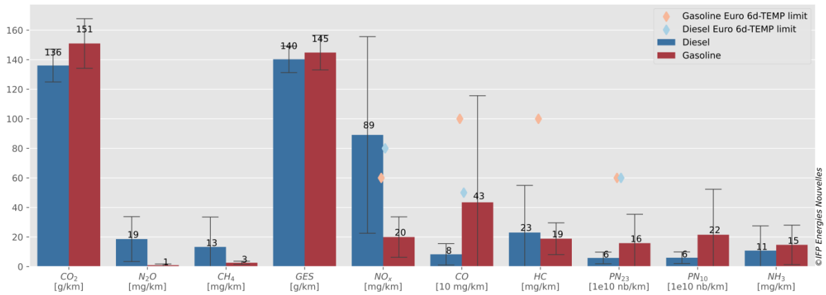
Figure 1 : Comparison of the average emissions of gasoline and diesel vehicles selected on the experimental protocol. Taking into account the impact of regeneration of diesel particulate filters. Measurements of N 2 O, CH 4 , GES, HC and PN10 on the scope of the dynamometer tests only. Error bars represent the standard deviation of each measurement sample.
