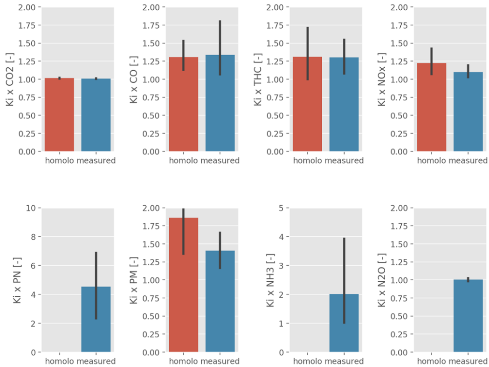
Figure 32 : Comparison of excess emission factors linked to periodic regeneration of pollution control systems
