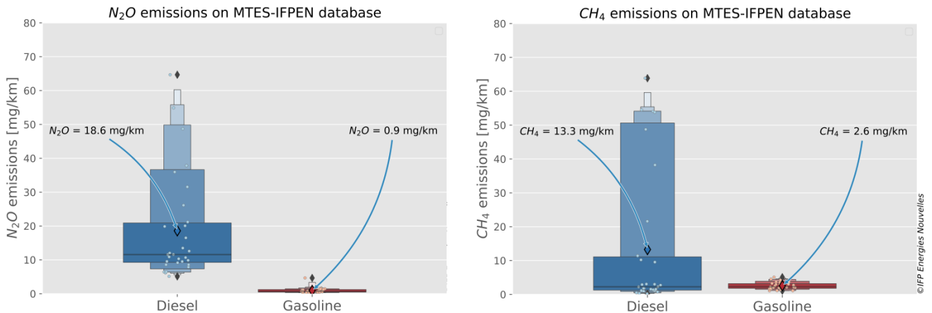
Figure 8 : Comparison of N_2O and CH_4 emissions from gasoline and diesel vehicles on the laboratory test scope (chassis dynamometer and climatic chassis dynamometer)
