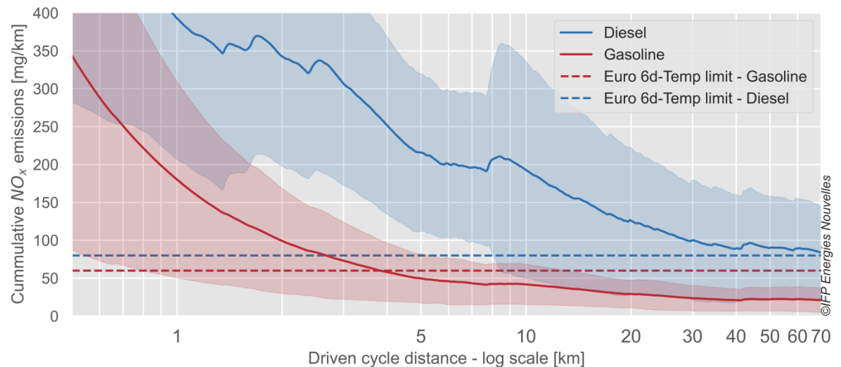
Figure 3 : Comparison of the evolution of cumulative NO x emissions as a function of the distance on the RDE test between gasoline and diesel vehicles (thick lines). The colored areas represent the standard deviation.
