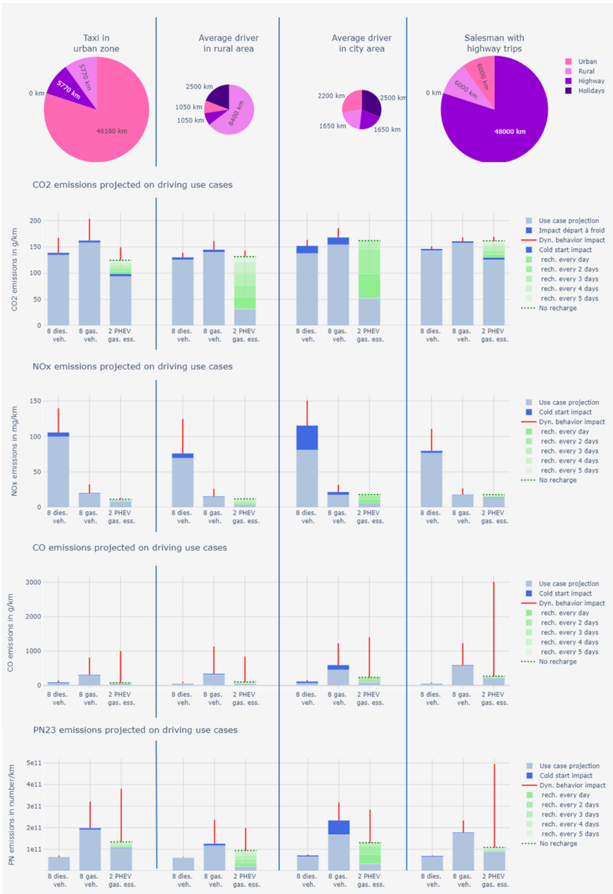
Figure 29 : Comparison of average emissions of CO 2 , NO x , CO and PN 23 projected on uses for diesel and gasoline combustion vehicles, and gasoline PHEV vehicles
