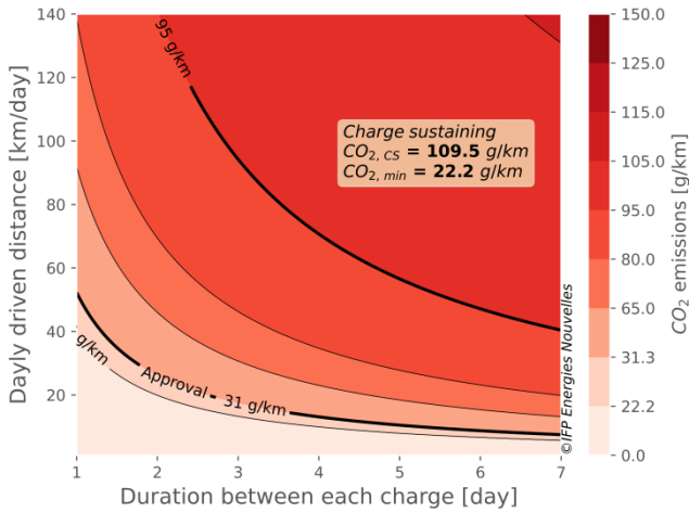
Figure 20 : CO 2 emissions of the PHEV vehicle depending on the frequency of recharging and the length of daily journeys. The approved CO 2 score is also shown (Approval). The considered scope does not include climatic tests which will be treated separately in this document.
