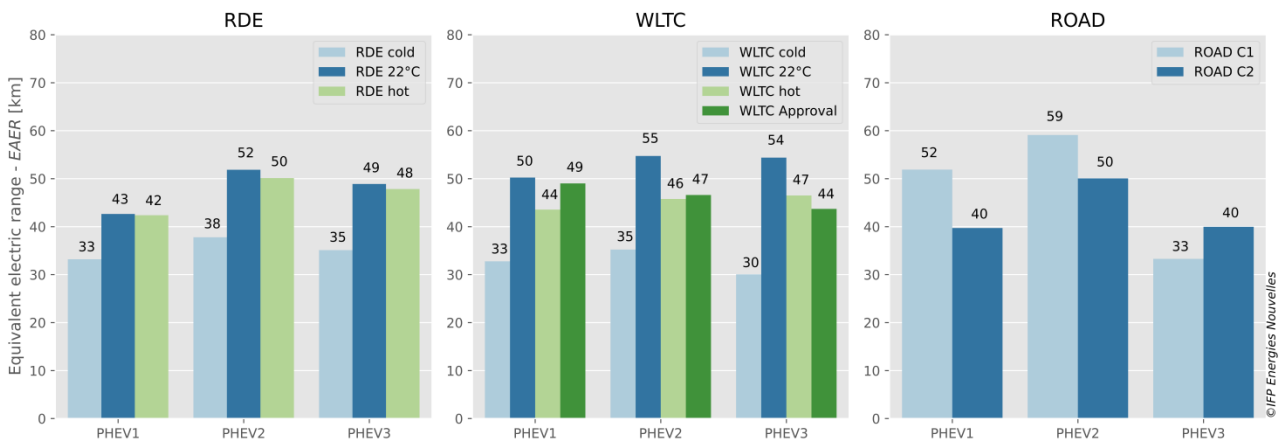
Figure 24 : Recalculated electrical equivalent range of the three PHEV vehicles of the study by type of test. The entire experimental perimeter is considered.
