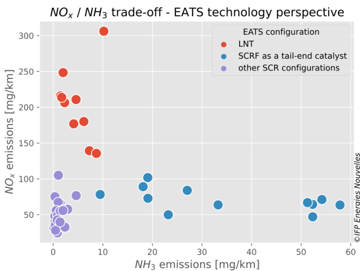
Figure 13 : Compromise of NH_3 and NO_x emissions in a NO_x treatment technology benchmark (each point represents the final cumulative score of a diesel vehicle test).
