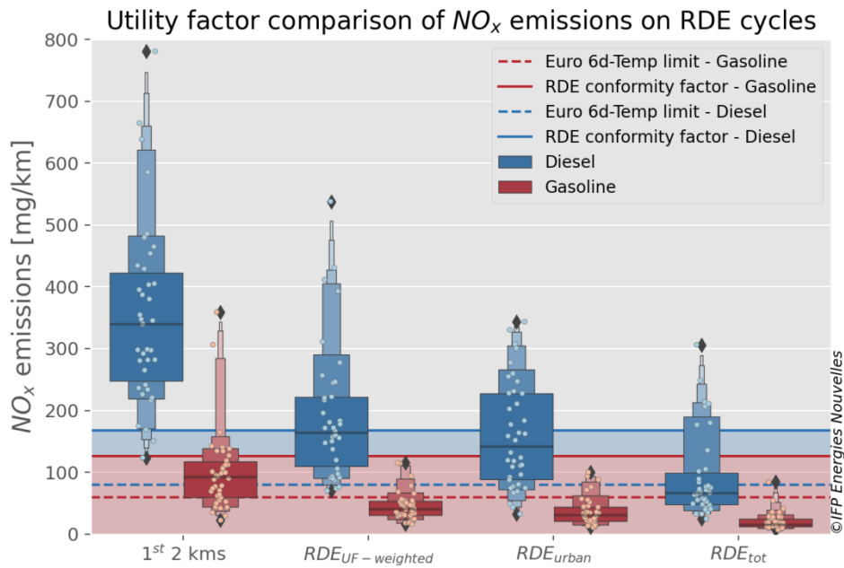
Figure 28 : NO_x emissions on full RDE tests, urban or weighted by actual use.
