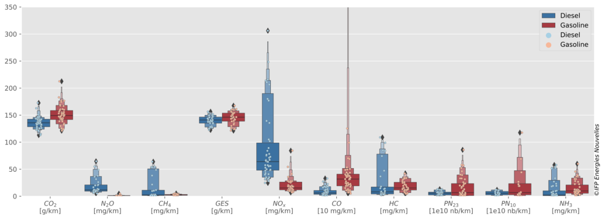
Figure 2 : Distribution of the emission levels of gasoline and diesel vehicles selected on the experimental protocol. Taking into account the impact of regeneration of diesel particulate filters. N 2 O, CH 4 , GES, HC and PN10 within the scope of the dynamometer tests only. Each point represents one test. The horizontal line represents the median of the sample. The most centrally located box extends from the 1st quartile (the 1st 4-quantile) to the 3rd quartile. The boxes, successively narrower than those which precede them, are delimited incrementally by the 8-quantiles, the 16-quantiles, the 32-quantiles and so on up to the extreme values of the data sample.
