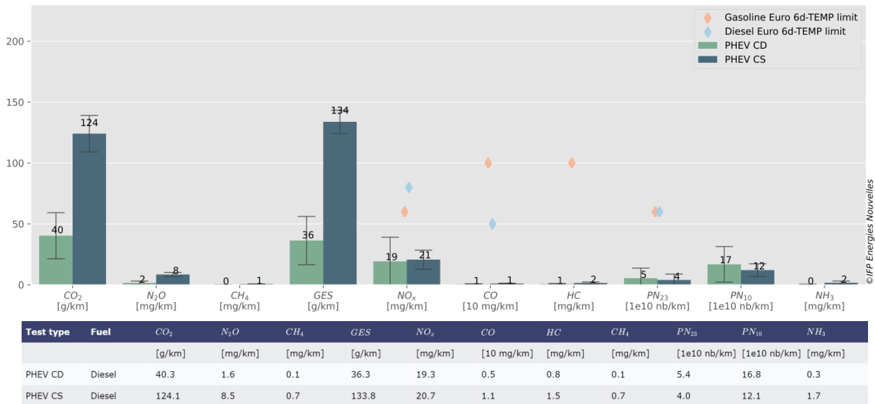
Figure 22 : Comparison of the mean emissions in CS and CD mode of the diesel plug-in hybrid vehicle selected on the experimental protocol.
