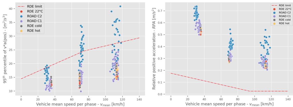
Figure 5 - Projections of the severity criteria of the RDE standard for each trial in the study; each point represents one of the 3 phases of a test (urban, rural and highway). The dotted red line describes the limit of the RDE standard.
