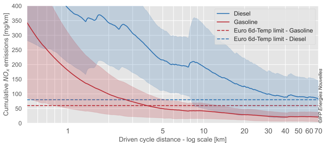
Figure 27 : Evolution of cumulative NO x emissions as a function of the distance on the RDE test
