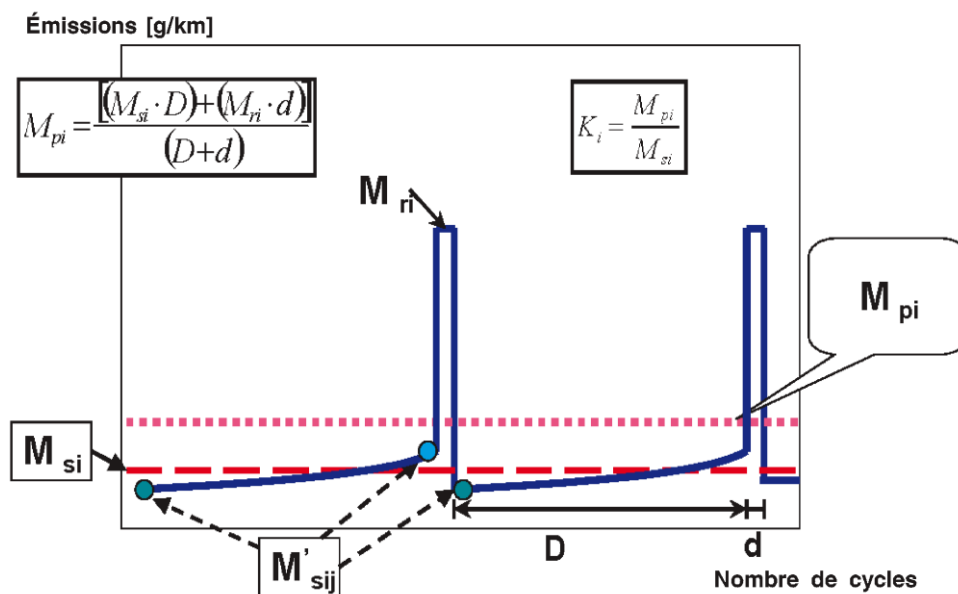
Figure 31 - Illustration of the method of controlling the emissions of a vehicle equipped with a periodically regenerating system - OJ of EU Commission reg. 2017-1151 supplementing reg. EC n ° 715-2007, p.536
