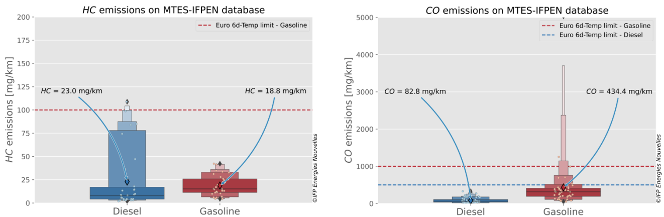
Figure 12 : Comparison of HC and CO emissions from gasoline and diesel vehicles on: laboratory tests for HC , the full scope of the study for CO
