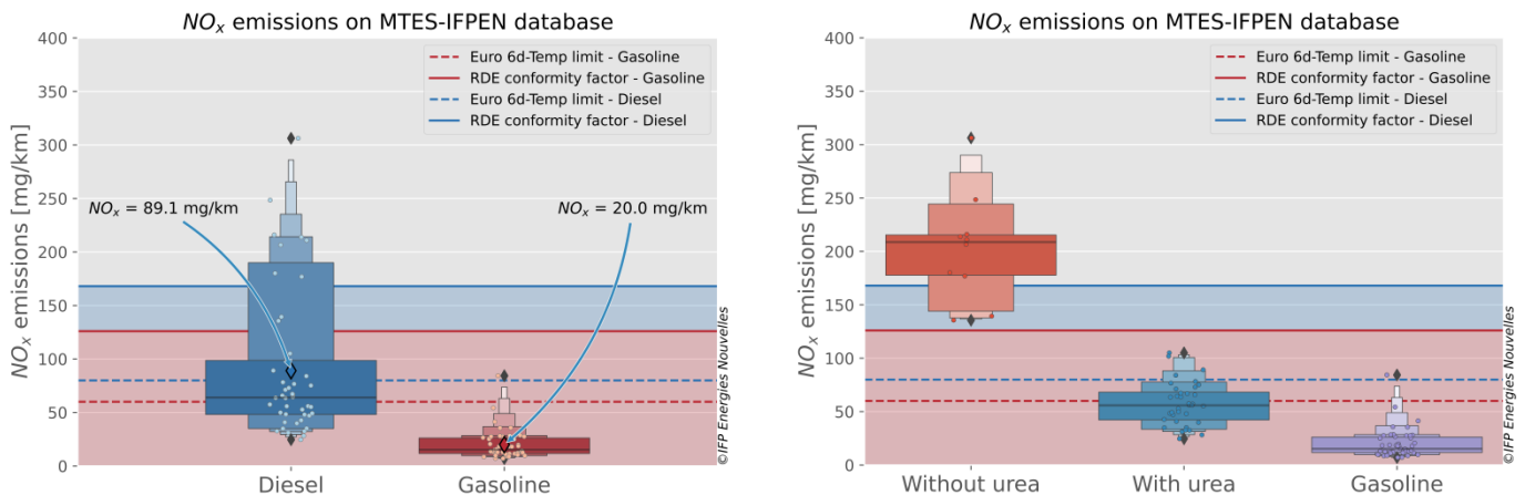
Figure 10 : Comparison of NO_x emissions from gasoline and diesel vehicles over the full scope of the study
