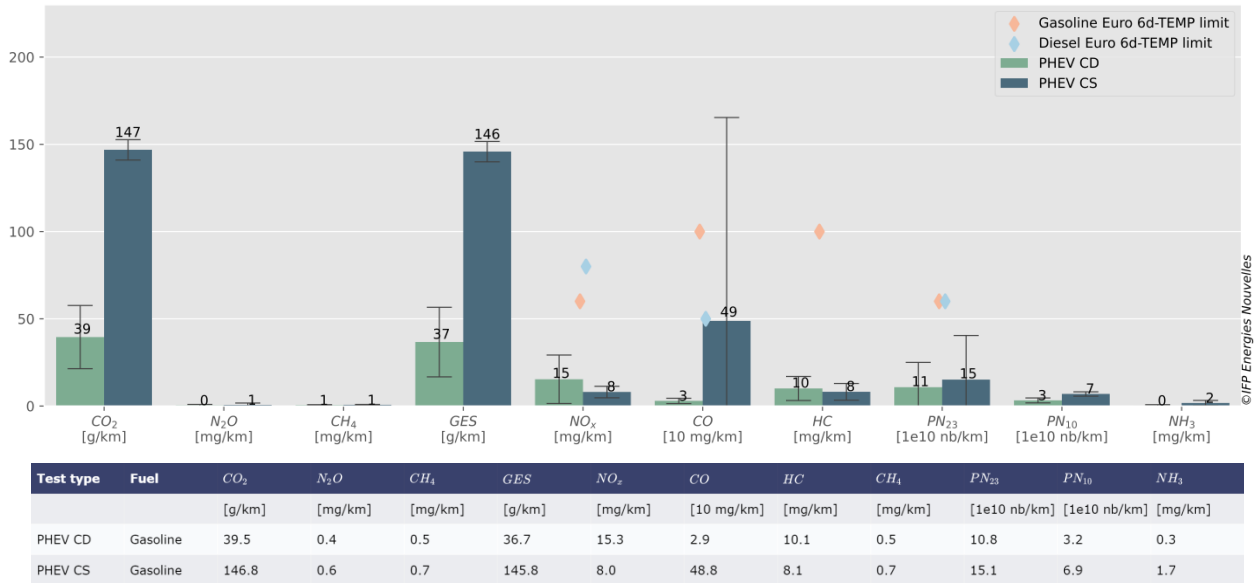
Figure 21 : Comparison of the average emissions in CS and CD mode of the gasoline plug-in hybrid vehicle selected on the experimental protocol.
