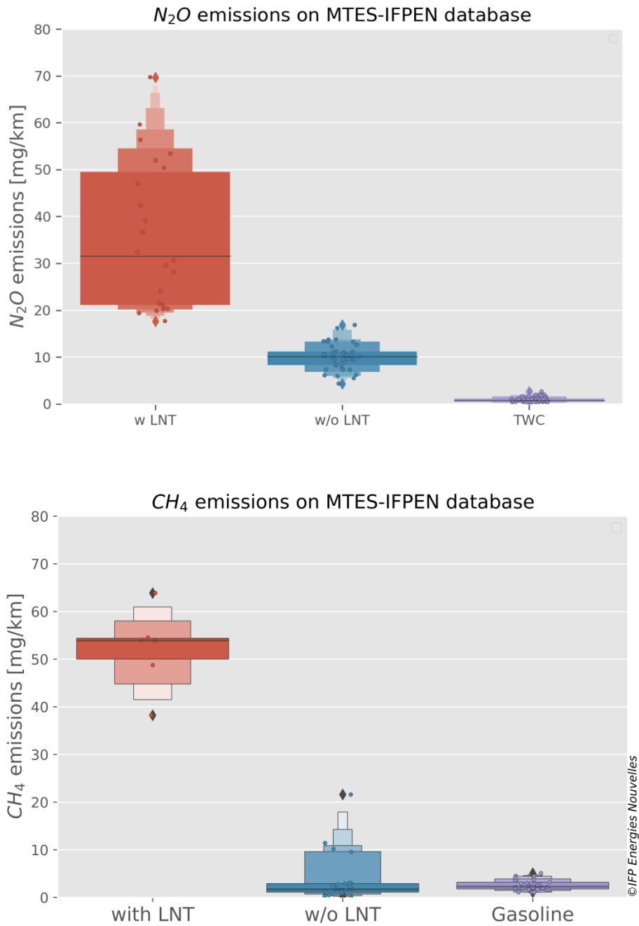
Figure 33 : Comparison of N 2 O and CH 4 emissions according to the types of pollution control of diesel and gasoline vehicles.
