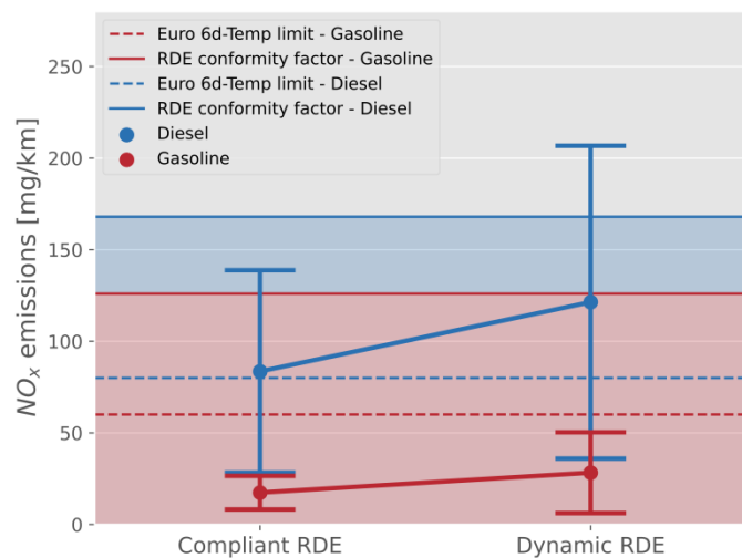
Figure 17 : Driving style sensitivity of NOx emissions on the experimental scope of the RDE road tests
