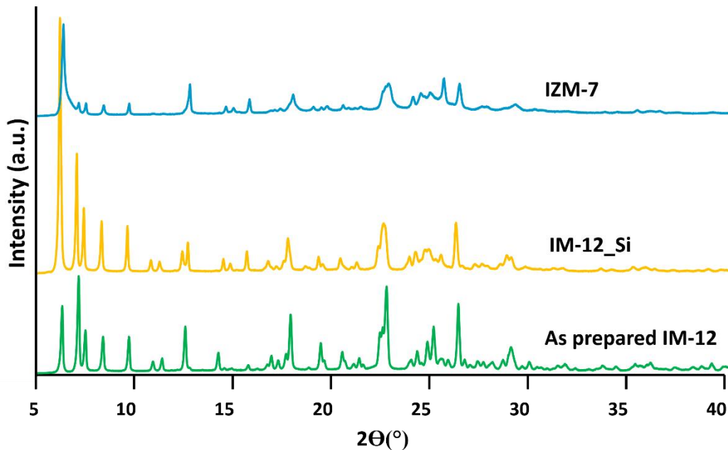
Figure 1: XRD patterns of as prepared IM-12, IM-12 treated with \text{SiCl}_4 (IM-12_Si) and IZM-7.
