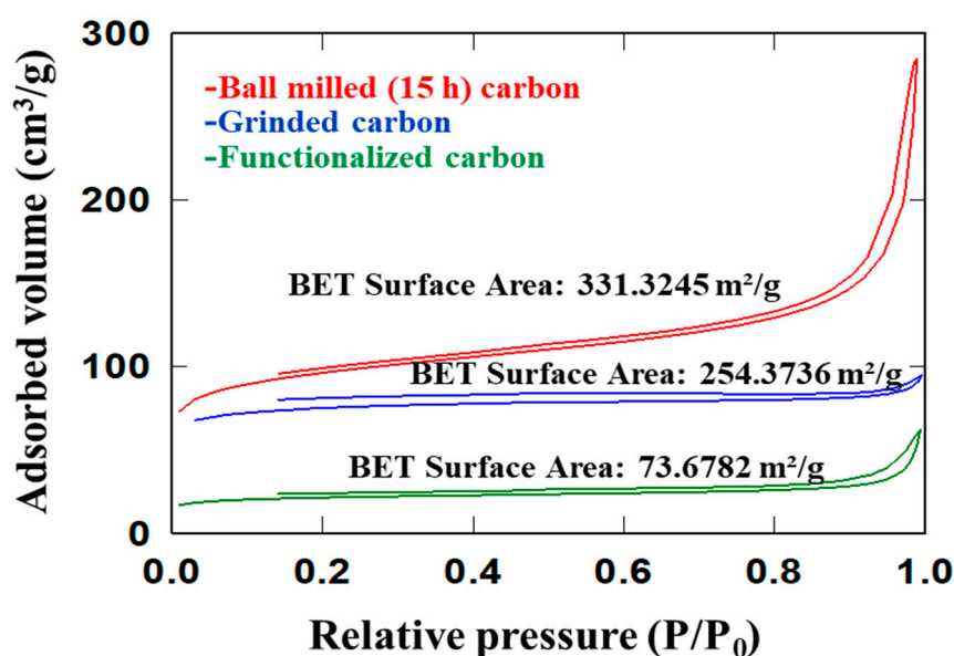
Figure 6. Nitrogen adsorption/desorption BET isotherms of the ground, ball-milled (15 h), and functionalized date carbon.
