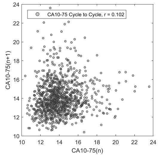
Figure 30 Case 2: Cycle-to-cycle correlation of CA10-75, \lambda=1.83 , Experimental data
