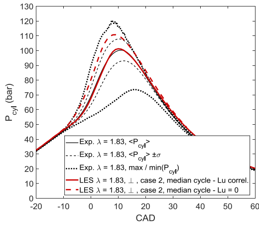
Figure 17 Effect of stretch on the in-cylinder pressure. Red line, CA50 median cycle (lean burn case 2); red dashed line, same cycle whose combustion phase has been calculated setting Lu to 0mm.
