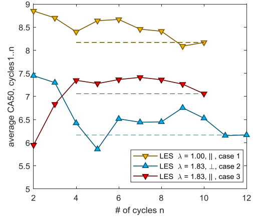
Figure 25 Mean CA50 for cycles' sets of increasing size. Orange triangles: LES case 1 (stoichiometric, || configuration); blue triangles, LES case 2 (lean, ⊥ configuration); red triangles, LES case 3 (lean, || configuration).
