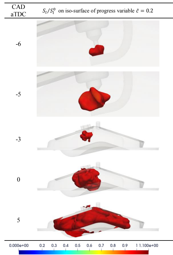
Figure 31 Case 1, evolution of flame propagation represented by Iso-surface of progress variable \tilde{c} = 0.2 , colored by S_t/S_t^0
