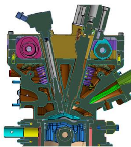
Figure 9 Cross section of engine's head-combustion chamber in the tumble plane
