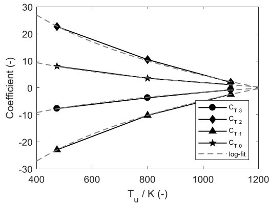
Figure 5 c_{T,i} coefficients as a function of T_u : star, c_{T,0} ; triangle: c_{T,1} ; diamonds: c_{T,2} ; dot: c_{T,3} .
