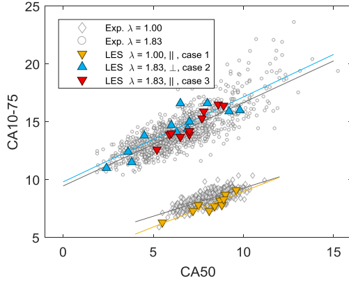
Figure 16 CA10-75 vs CA50, Gray diamonds: experimental data \lambda = 1.0 ; Gray dots: experimental data \lambda = 1.83 ; orange triangles: LES case 1 (stoichiometric, \parallel configuration); blue triangles: LES case 2 (lean, \perp configuration); red triangles: LES case 3 (lean, \parallel configuration).
