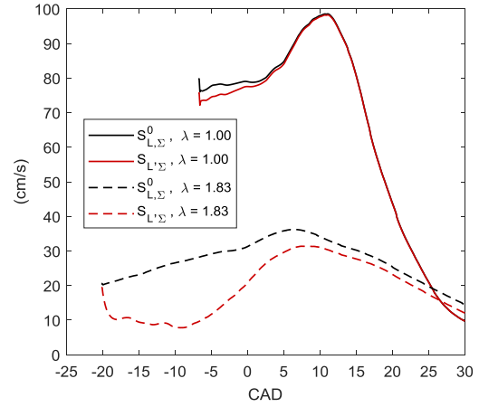
Figure 19 Evolution of the un-stretched laminar flame speed S_L^0 (black) and the effective laminar flame speed S_L (red) on the flame front. Solid line: Stoichiometric case 1; dashed line: lean burn case 2. For both cases, the median cycle in terms of CA50 is considered.
