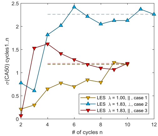
Figure 26 Unbiased standard deviation of CA50 for cycles' sets of increasing size. Orange triangles: LES case 1 (stoichiometric, || configuration); blue triangles, LES case 2 (lean, ⊥ configuration); red triangles, LES case 3 (lean, || configuration).
