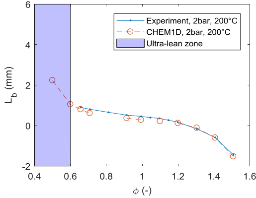
Figure 2 Burned gas Markstein length L_b as a function of \phi for an iso-octane/air mixture at 2 bar and 473 K. Solid line: experiment, red dots: calculated Markstein lengths
