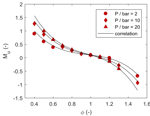
Figure 8 Comparison between CHEM1D calculated fresh gas Markstein number \mathcal{M}_u and the proposed correlation (continuous line) at T_u = 800 K, P/\text{bar} \in \{2, 10, 20\} and 0.4 \leq \phi \leq 1.5 : dots, P = 2 bar; diamonds, P = 10 bar; triangles, P = 20 bar
