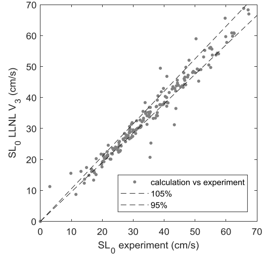
Figure 27 Correlation graph simulation versus experiment for the un-stretched laminar flame speed.
