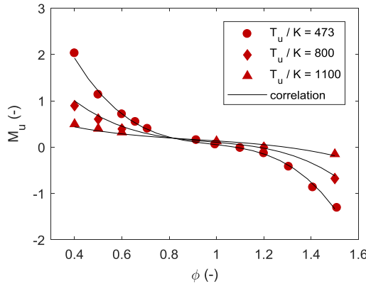
Figure 7 Comparison between CHEM1D calculated fresh gas Markstein number \mathcal{M}_u and the proposed correlation (continuous line) at P = 2 bar, T_u/K \in \{473, 800, 1100\} and 0.4 \leq \phi \leq 1.5 : dots, T_u = 473 K; diamonds, T_u = 800 K; triangles, T_u = 1100 K.
