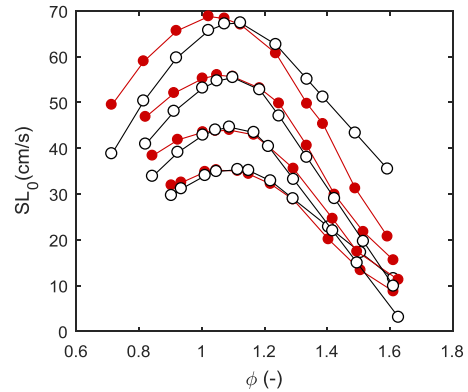
Figure 27 Correlation graph simulation versus experiment for the un-stretched laminar flame speed.
