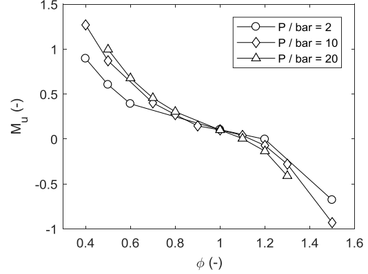
Figure 6 Fresh gas Markstein number \mathcal{M}_u as a function of \phi at T_u = 800 K: dots, P = 2 bar; diamonds, P = 10 bar; triangles, P = 20 bar
