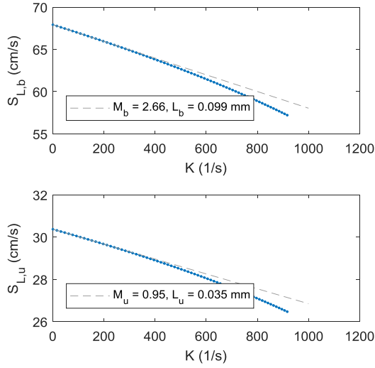
Figure 1 Burned gas laminar flame speed S_{Lb} (above) and fresh gas laminar flame speed S_{Lu} (below) for C_8H_{18} /air mixture as function of stretch, \lambda = 1.83 , P = 31 bar, T = 745 K. For each case is plotted the regression line whose slope is the Markstein length: L_u in fresh gas and L_b in burned gas.
