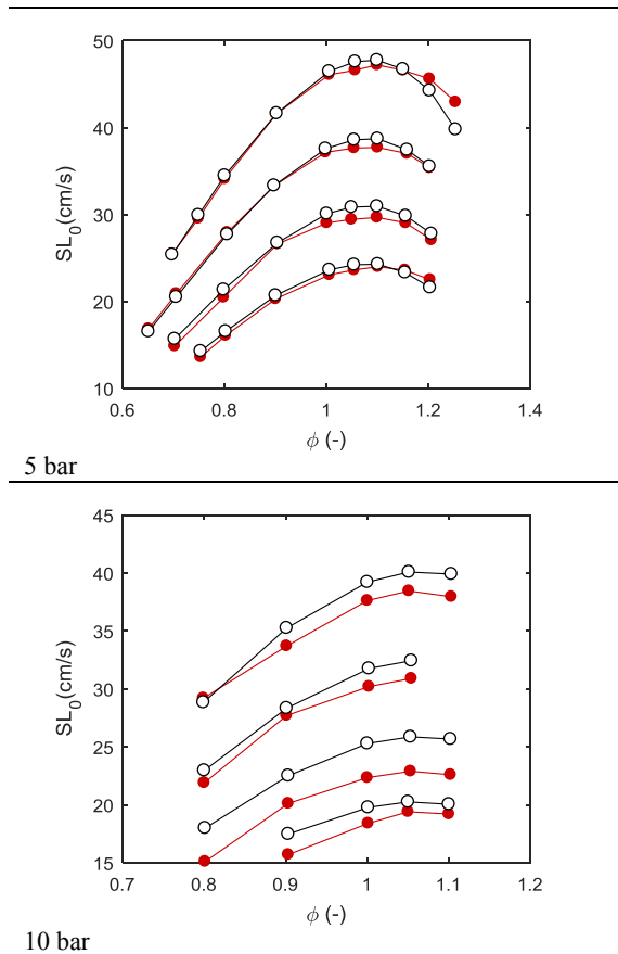
Figure 28 Comparison between calculated laminar flame speeds and experimental results at 1, 2, 5 and 10 bar. Red: experiment, black: calculation. T=323K (lowest curve), 373K, 423K, 473K (highest curve)
