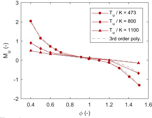
Figure 4 Fresh gas Markstein number \mathcal{M}_u as a function of \phi at P = 2 bar: dots, T_u = 473 K ; diamonds, T_u = 800 K ; triangles, T_u = 1100 K; dashed line, best fit 3 rd order polynomial
