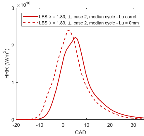
Figure 18 Effect of the stretch on the heat release rate per unit of volume. Continuous line, CA50 median cycle (lean burn case 2); dashed line, same cycle whose combustion phase has been calculated setting Lu to 0mm.
