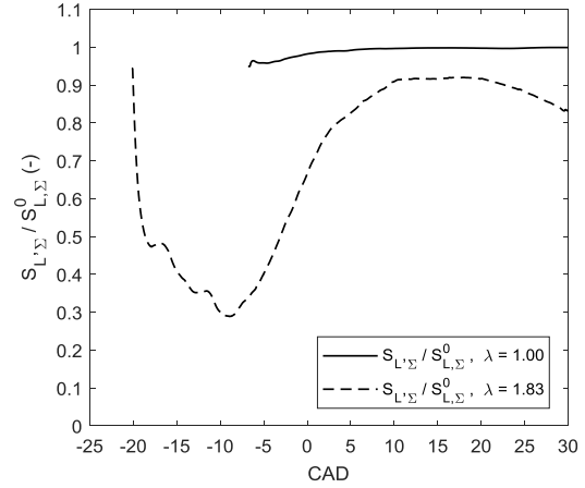
Figure 20 Evolution of S_{L,S}/S_{L,S}^0 . Solid line: Stoichiometric case; dashed line: lean burn case 2 (same cycles as in Figure 19).
