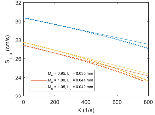
Figure 3 Stretched Laminar flame speed and Markstein length for fresh gas. Blue: iso-octane, \lambda = 1.83 ; red: iso-octane, \lambda = 1.89 ; orange: surrogate, \lambda = 1.89 . P = 31 bar, T = 745 K in all 3 cases
