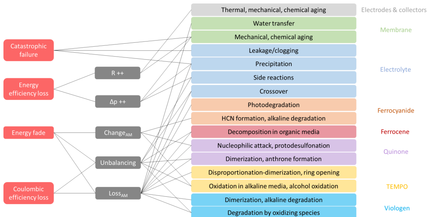
Figure 8 Performances' degradations and their causes in aqueous organic redox flow batteries
