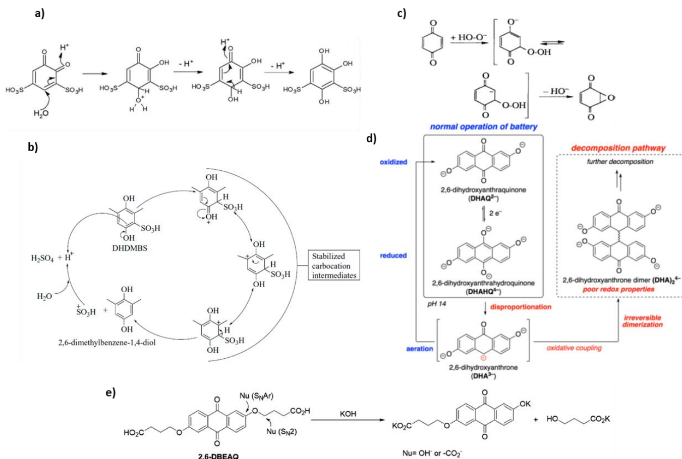
Figure 4 Quinones degradations reactions
