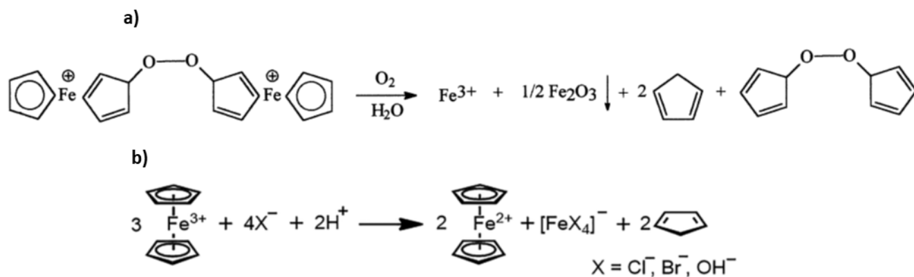
Figure 3 Ferrocene degradations reactions
