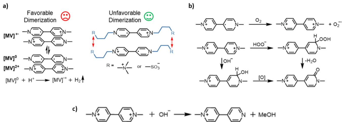
Figure 6 Viologen degradation reactions [8]
