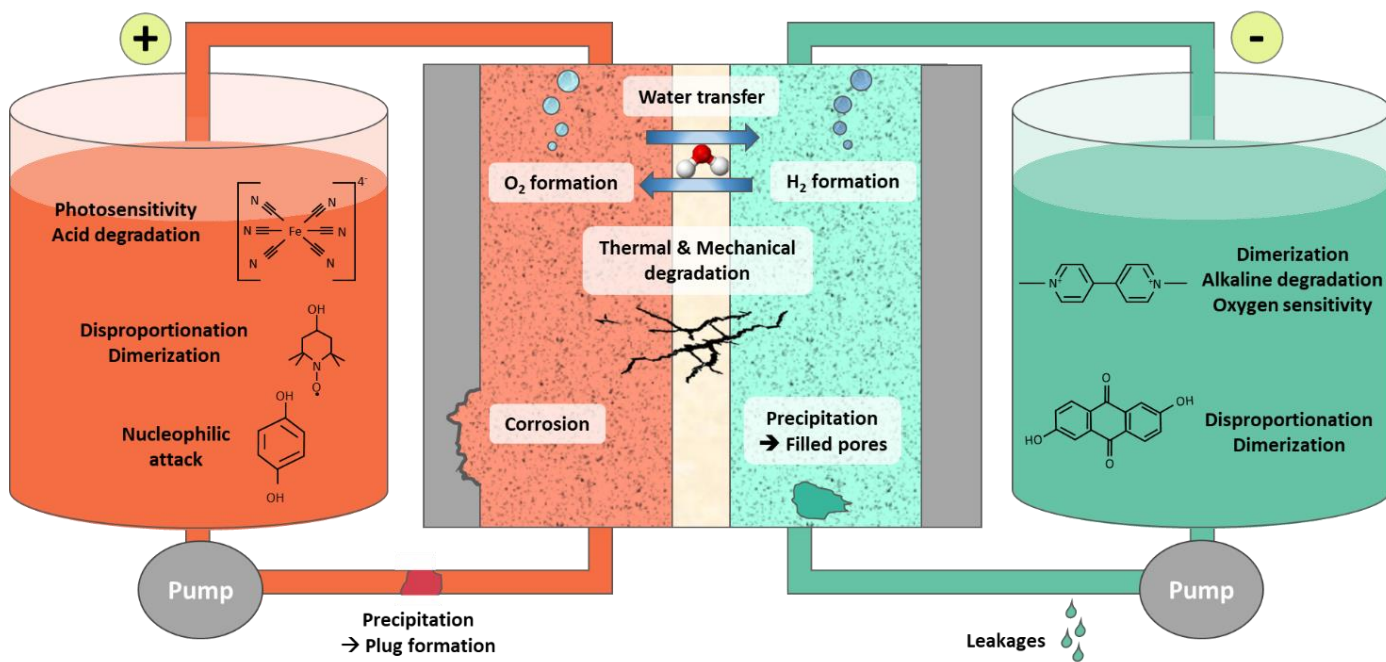
Figure 7 Main degradation mechanisms in aqueous organic redox flow batteries
