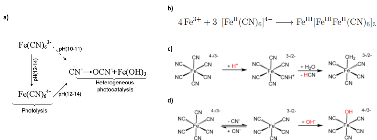
Figure 2 Ferrocyanide degradations reactions
