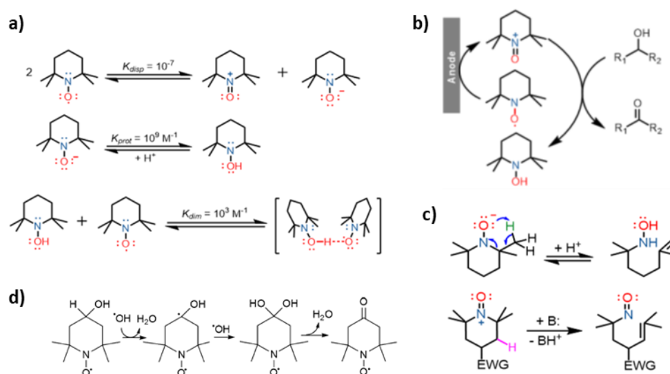
Figure 5 TEMPO degradations reactions
