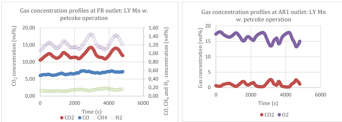
Figure 7: Profiles of gas concentrations at outlet of FR and AR1 during a reference test with solid fuel an LY Mn ore
