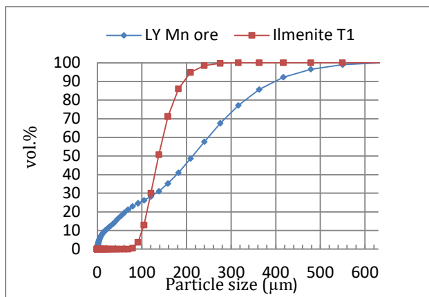
Figure 2: Particle Size Distribution of OCs (red: ilmenite, blue: LY Mn ore)
