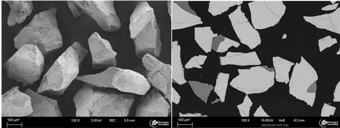
Figure 14: SEM images of ilmenite T1 (left: direct observation; right: polished cross-section)
