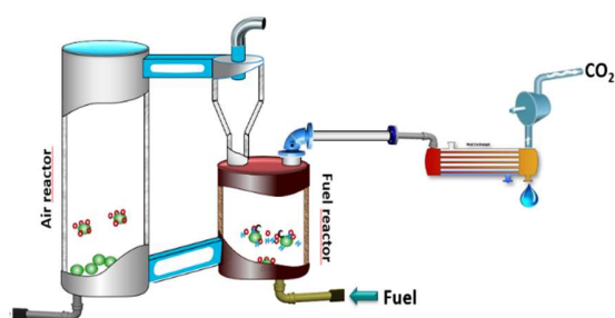
Figure 1: Diagram of chemical looping combustion process
