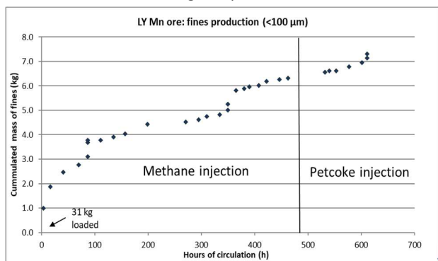
Figure 16: Mass of fines recovered as a function of circulation time during LY Mn campaign (Petcoke combustion was not performed on a continuous basis).
