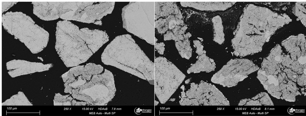
Figure 15: SEM cross-section analysis of Ilmenite during methane activation (left: after 34h; right: after 108h)
