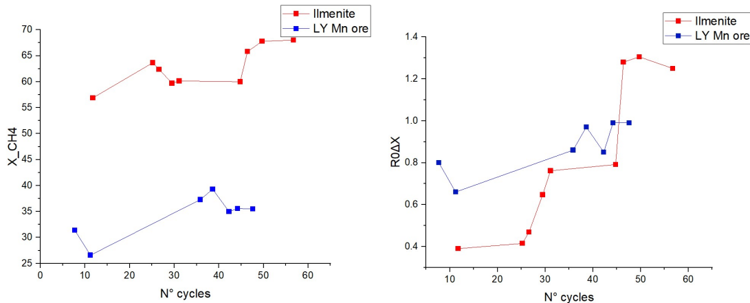
Figure 5: Evolution of methane conversion and R_0\Delta X during LY Mn ore activation cycles in comparison to Ilmenite T1 behavior
