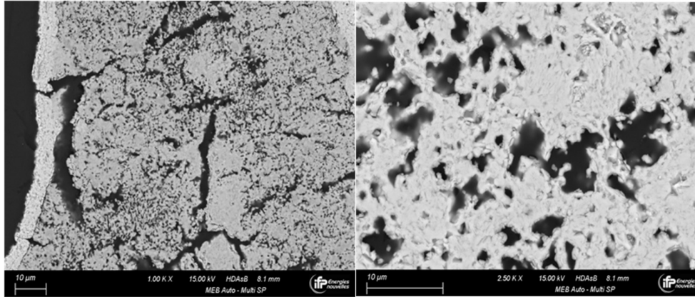
Figure 12: cross-section SEM images of LY-Mn ore powder after 52 hours of methane activation
