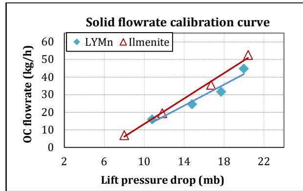
Figure 4 : Calibration curve of the solid flow rate in the unit over the pressure drop in the lift after AR2
