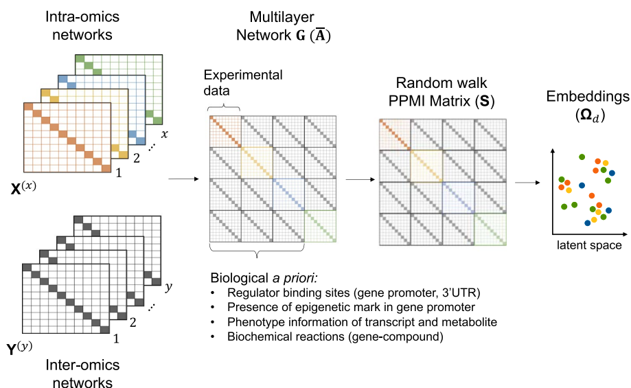
Fig. 2 Overview of BRANENET. Inputs ( X ) and ( Y ) are on the left. A multilayer network \bar{\mathbf{A}} is composed of intra- and inter-omics relationships. For \bar{\mathbf{A}} , the random walk-based PPMI matrix \mathbf{S} is computed. To obtain embeddings, \mathbf{S} is factorized and the final embeddings \Omega_d are obtained
