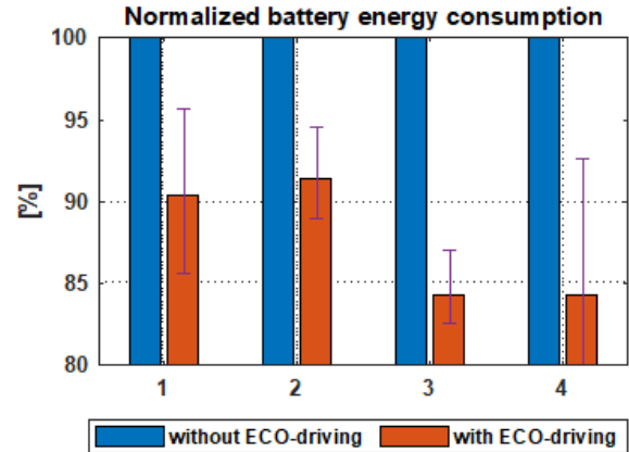
Figure 14: Battery energy consumption with and without ECO-driving for the two directions of the trip
