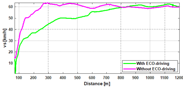
Figure 13: Zoom on an acceleration with and without ECO-driving
