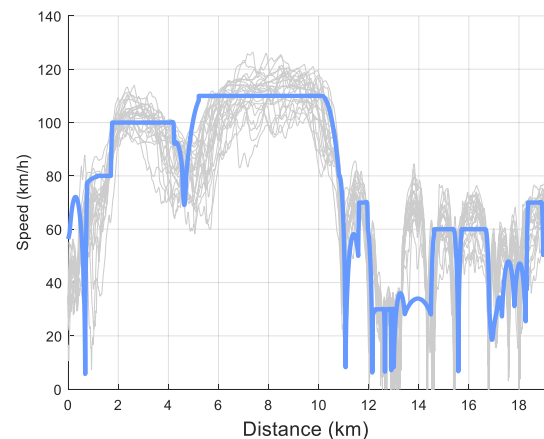
Figure 4: Driven (gray) and eco (blue) speed profile
