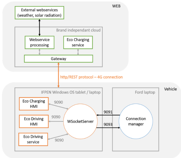
Figure 9: Implementation architecture
