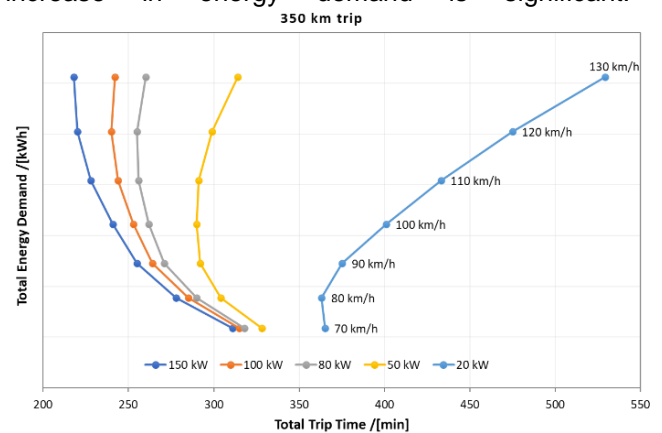
Figure 1: Dependency between available charging power, energy demand and trip time for a long distance trip
