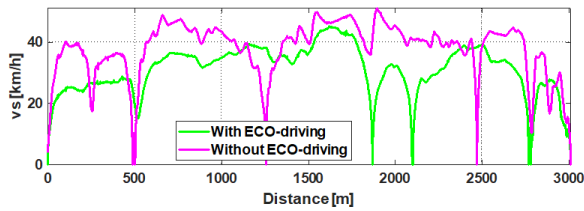
Figure 12: Urban route with and without ECO-driving
