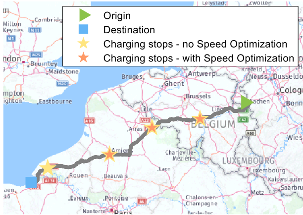
Figure 2: Mission profile between Aachen (Germany) and Deauville (France) (© 2022 HERE)
