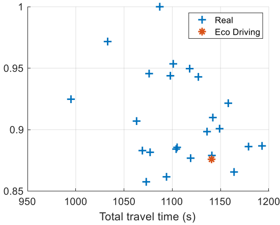
Figure 5: Normalized battery energy consumption according to the total travel time
