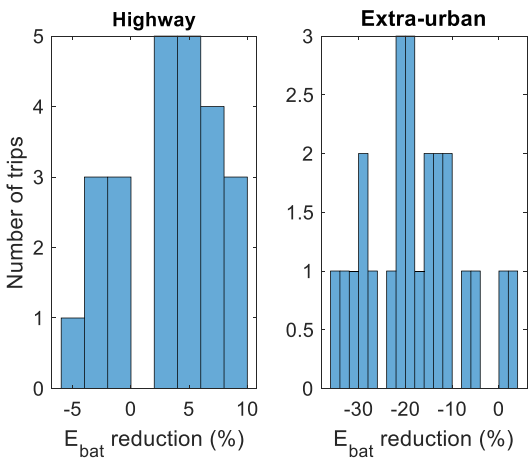
Figure 7: Battery energy reduction distribution according to route type
