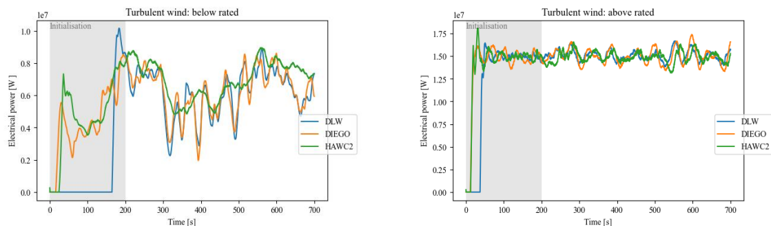
(a) Electrical power below rated wind speed (b) Electrical power above rated wind speed Figure 6: Electrical power curve comparisons below and above rated wind speed
