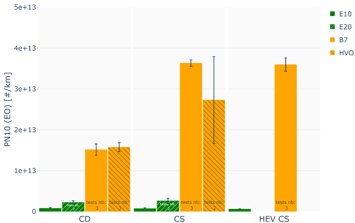
Figure 22 Comparison of engine-out PN10 emissions [#/km] measured on RDE cycles on chassis dyno for each fuel and mode.
