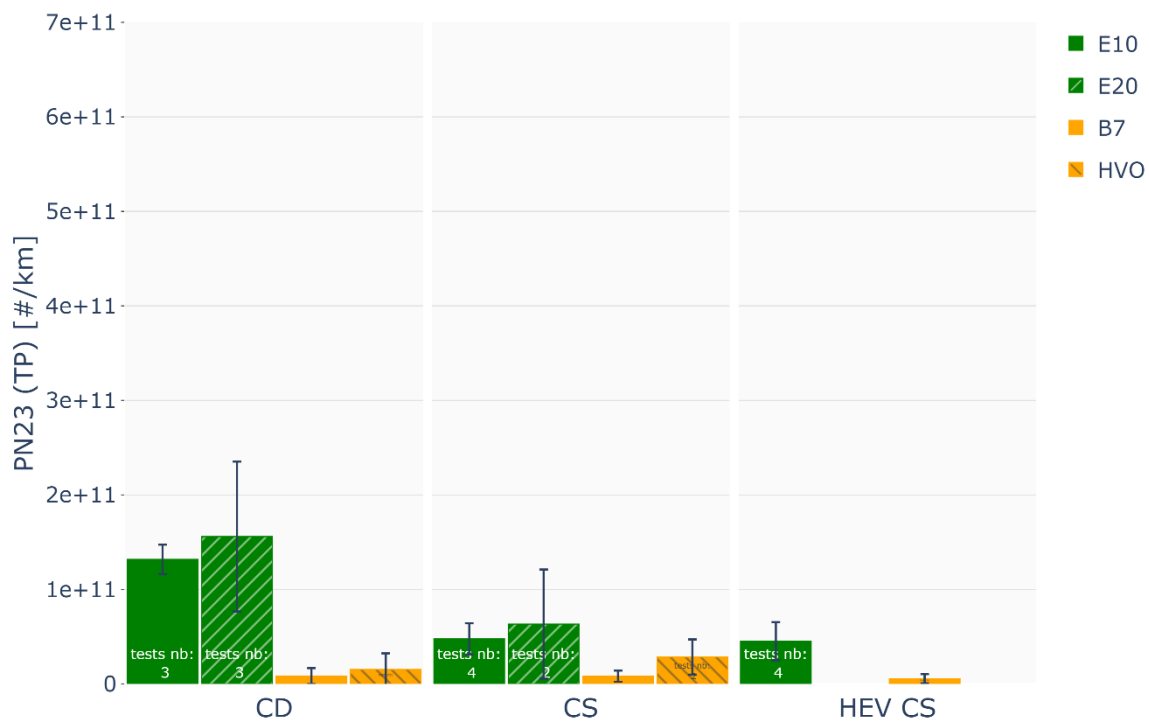
Figure 23 Comparison of tailpipe PN23 emissions [#/km] measured on RDE cycles on chassis dyno for each fuel and mode.
