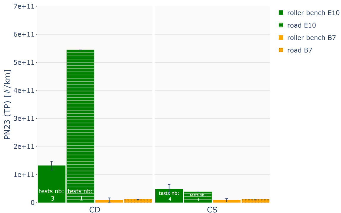
Figure 49 Comparison of tailpipe PN23 emissions [#/km] measured on RDE on-road and chassis dyno tests for each fuel and mode.
