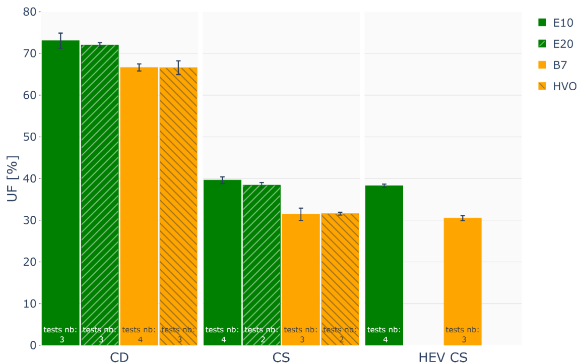
Figure 10 Comparison of Utility factor [%] measured on RDE cycles on chassis dyno for each fuel and mode.
