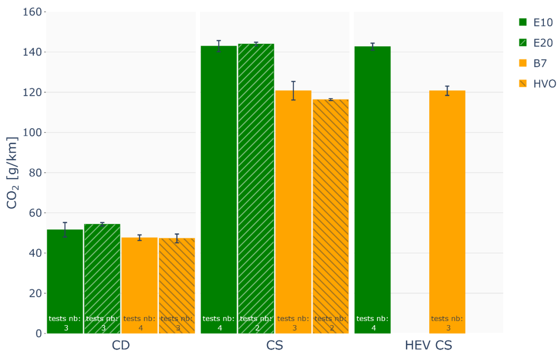
Figure 11 Comparison of tailpipe CO 2 emissions [g/km] measured on RDE cycles on chassis dyno for each fuel and mode.
