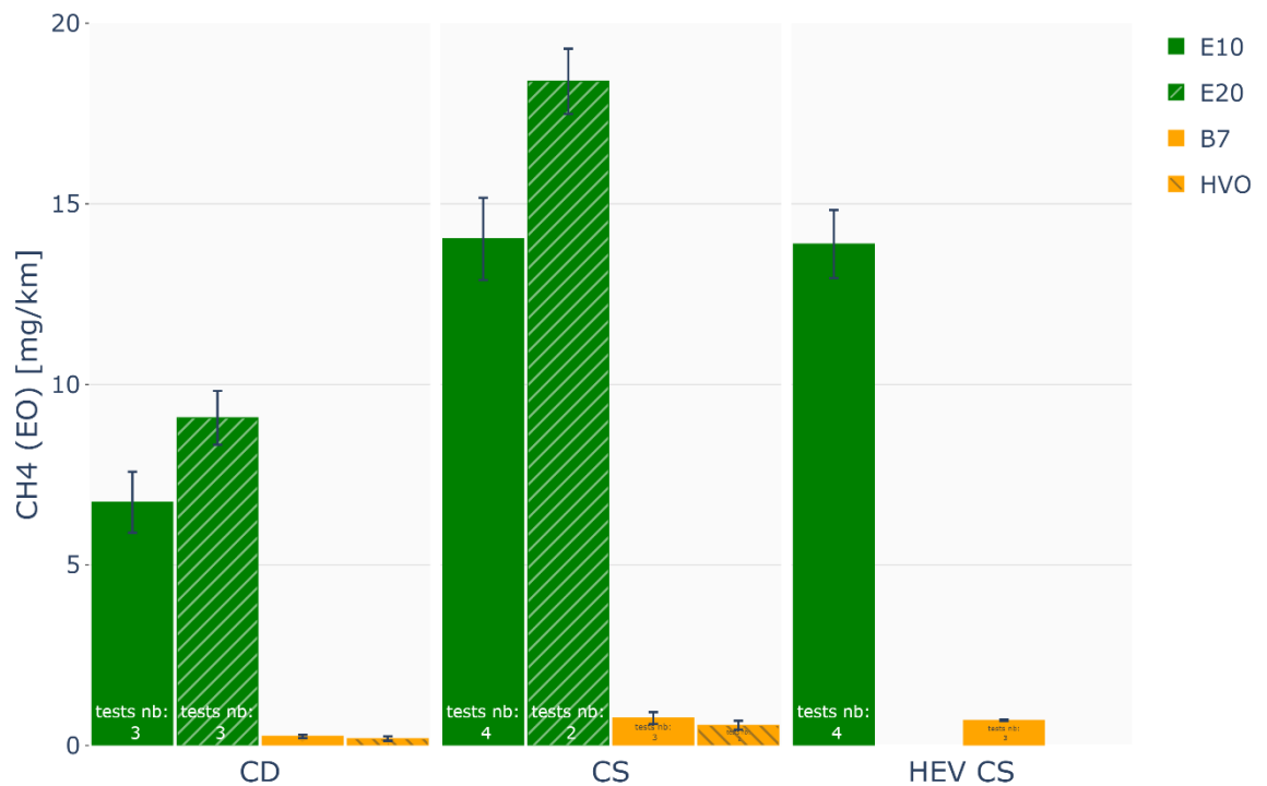
Figure 14 Comparison of engine-out CH 4 emissions [mg/km] measured on RDE cycles on chassis dyno for each fuel and mode.
