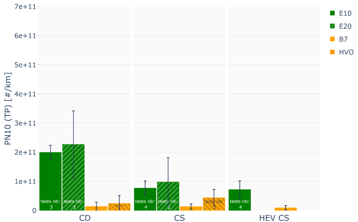
Figure 24 Comparison of tailpipe PN10 emissions [#/km] measured on RDE cycles on chassis dyno for each fuel and mode.
