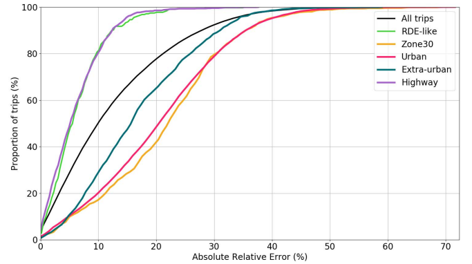
Fig. 9. Cumulative distribution of the absolute relative error for all trips and for each road type, for the subset of trips containing more than 90% of this specific road type. RDE-like trips are also recorded.
