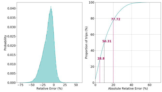
Fig. 8. Histogram of the relative error (left). Cumulative distribution of the absolute relative error (right). Significant absolute relative error thresholds (5, 10 and 20 percent) are highlighted with purple lines and the corresponding proportion of trips satisfying the thresholds are indicated in bold.
