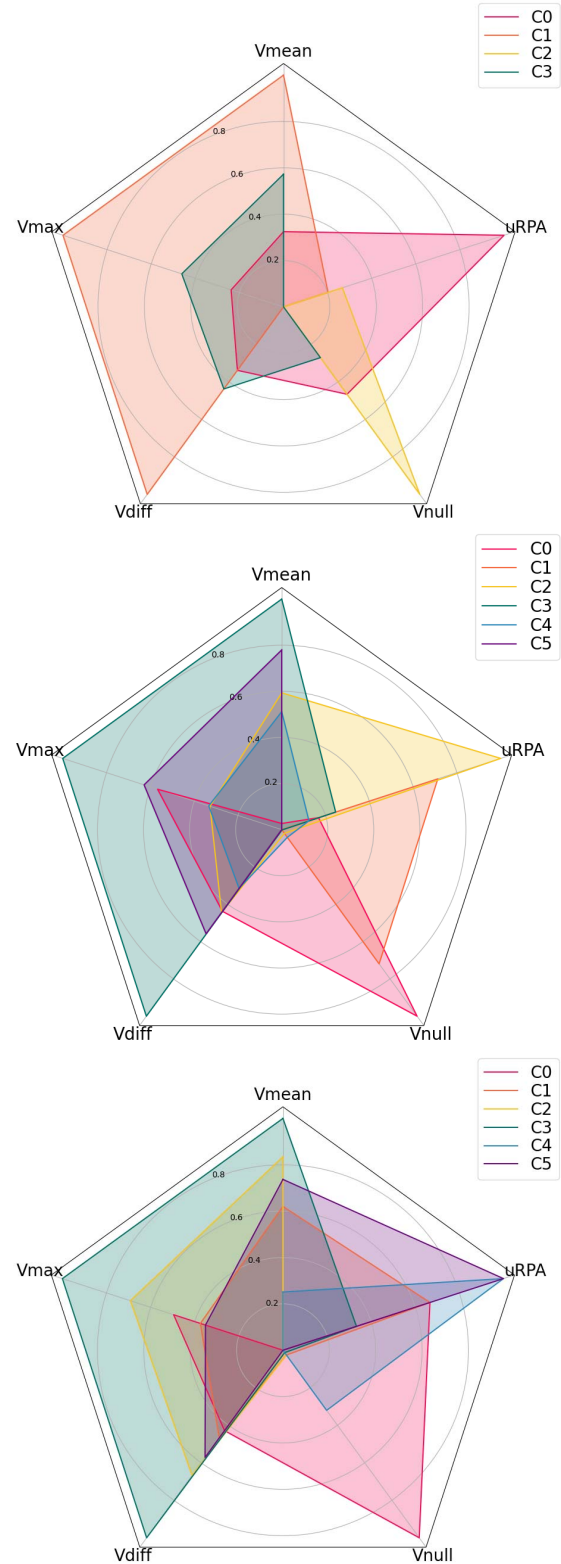
Fig. 10. Radar plot for comparing centroids of clusters obtained on URBAN (top), \chi -URBAN (middle) and HIGHWAY (bottom). Centroids are restricted to five descriptors ( v_{\text{mean}} , v_{\text{max}} , v_{\text{null}} , \bar{v}_{\text{diff}} and RPA_{\text{unweight}} ) and are normalized between 0 and 1 for a relative comparison between clusters.
