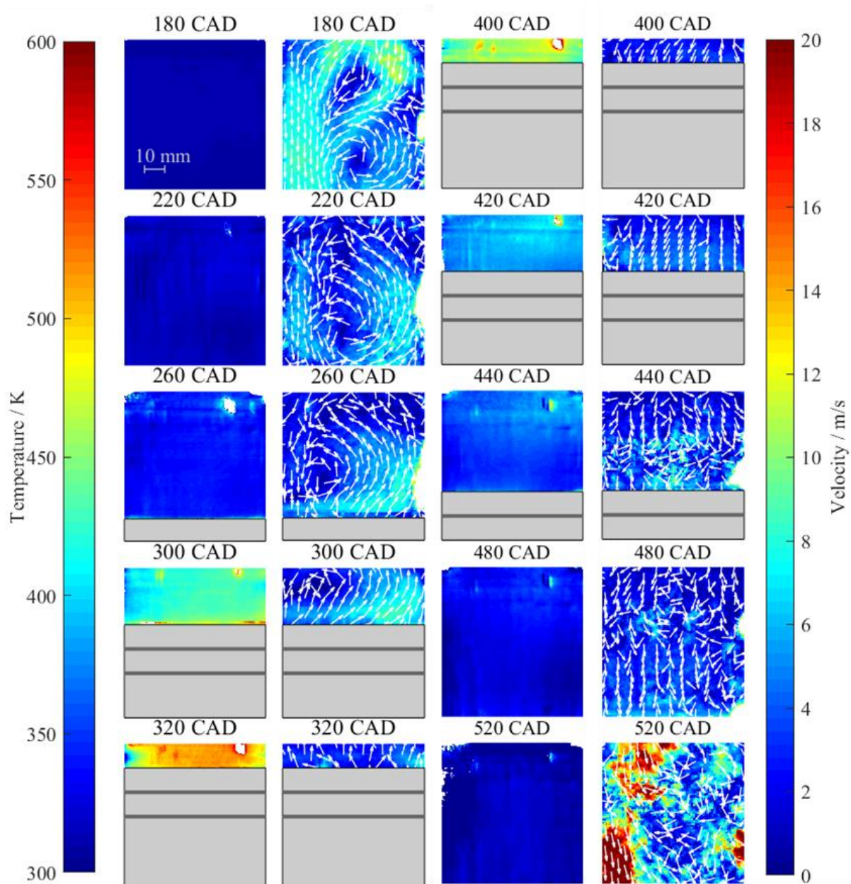
1 2 Figure 19: Simultaneous temperature and velocity fields from the operation condition “increased tumble”. The intake valves are 3 located on the top right, and the exhaust valve on the top left of the image. The flatfield correction is performed towards bottom 4 dead center of the reference condition. For improved visibility, only every second velocity vector is shown.
