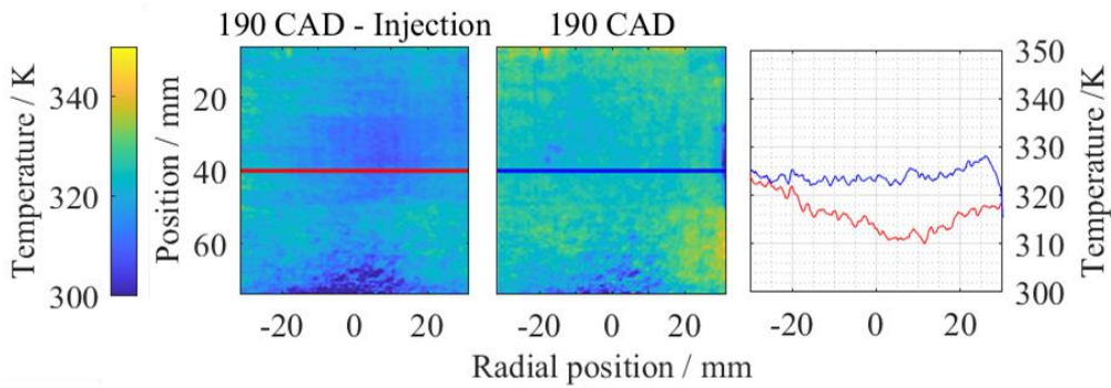
8 9 Figure 18: Average temperature field (left and center) of the in-cylinder gas and temperature profile (right) with and without fuel 10 injection. The reference temperature profile from motored operation (no fuel injection) is annotated in blue. The vertical position 11 is given relatively to the viewing plane shown in Figure 4.
