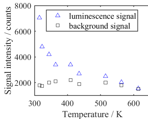
15 16 Figure 17: Luminescence and background signal intensities at increasing in-cylinder temperatures.
