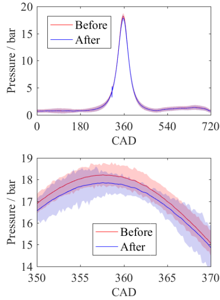
1 2 Figure 7: Pressure trace before and after dismounting and cleaning the optical engine under motored operation. Bottom: 3 enlargement around TDC. Transparent overlay: variation in pressure from 500 consecutive cycles. The mean pressure traces are 4 shown with a solid line.
