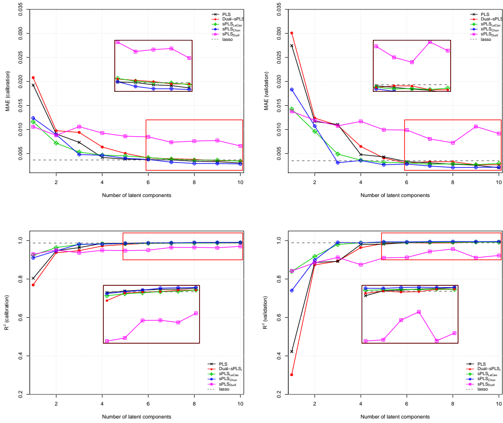
Figure B.10: Dual-sPLS 1 evaluation on real data D_{\text{NIR}} . MAE (top) and R^2 (bottom) values for calibration (left) and validation (right) with respect to the number of latent components derived from PLS, Dual-sPLS 1 , sPLS LeCao , sPLS Chun , sPLS Durif and lasso regressions.
