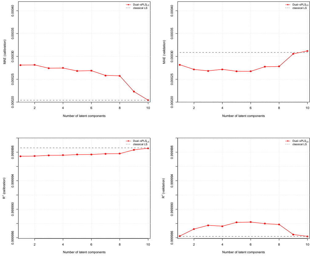
Figure B.11: Dual-sPLS LS evaluation on simulated data \overline{D}_{SIM} . MAE (top) and R^2 (bottom) values for calibration (left) and validation (right) with respect to the number of latent components derived from Dual-sPLS LS and least squares regressions.
