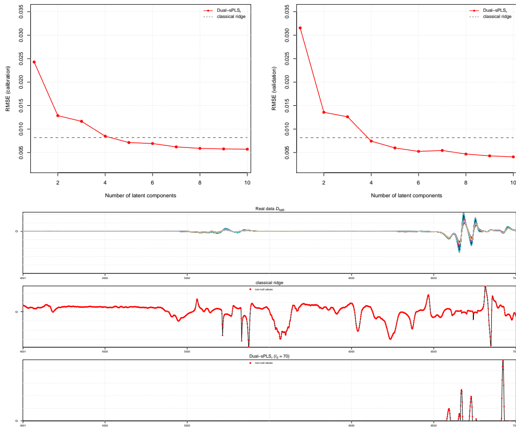
Figure 8: Dual-sPLS T evaluation on real data D_{\text{NIR}} . (Top) RMSE values for calibration (left) and validation (right) with respect to the number of latent components. (Bottom) From top to bottom: original data D_{\text{NIR}} , regression coefficients of ridge and Dual-sPLS T for five components.
