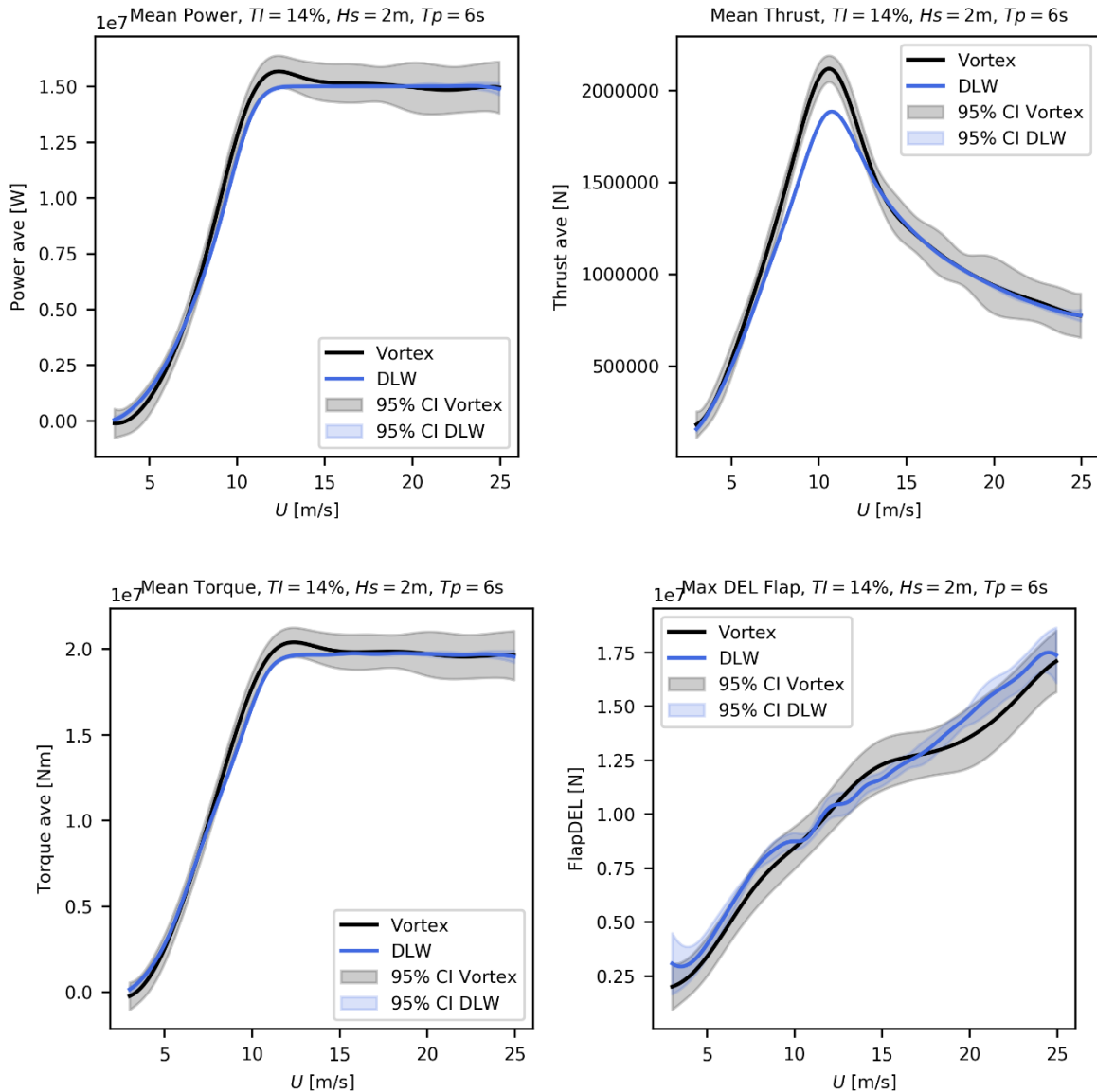
Figure 88: Power, Thrust, Torque, and DEL flap curves estimated with the metamodels calibrated from BEM simulations and Vortex simulations for a floating wind turbine for a TI = 14\% , H_s = 2m , Tp = 6s , \theta_{wind} = 195^\circ , \theta_{waves} = 165^\circ .
