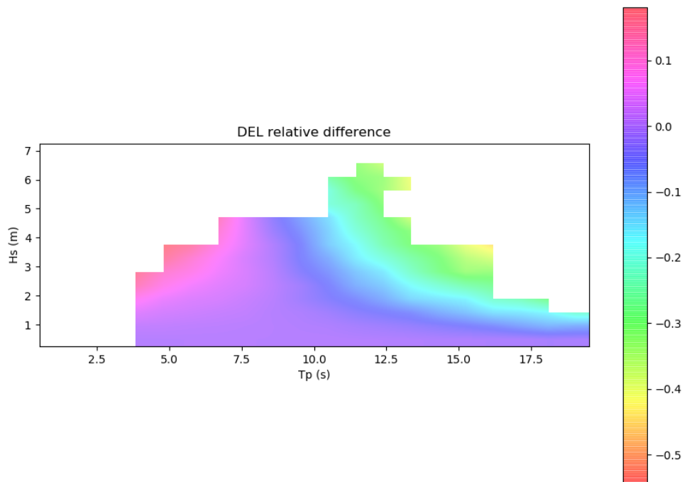
Figure 26: Water depth = 12.5m. DTU D=8.6m case. Relative DEL error between MCF and the Potential Flow theory (positive value means MCF produces higher DEL).
