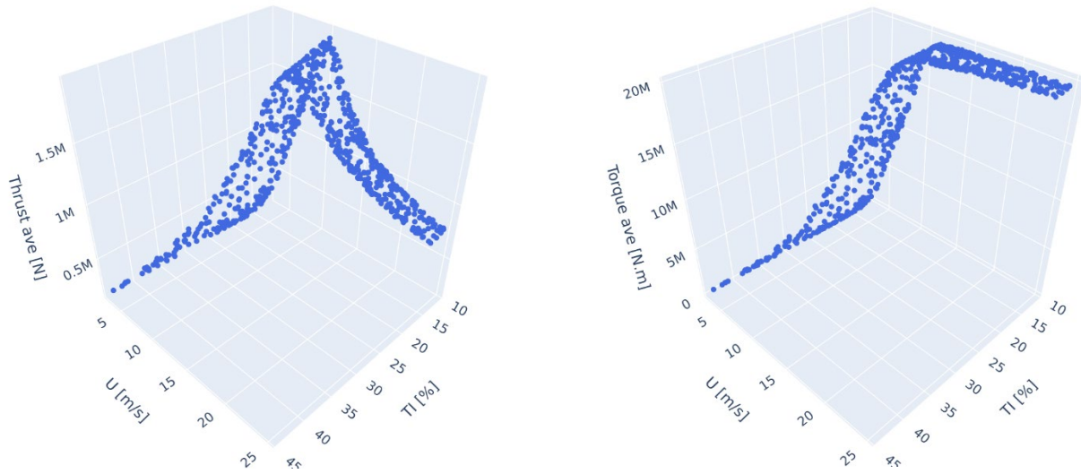
Figure 84. DLW BEM results for mean thrust (left) and mean torque (right) for South Brittany floating case
