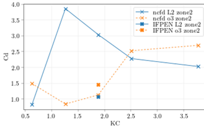
Figure 56: Drag coefficient for zone 2, with two different extraction methods. Sway imposed motions. KC varying.
