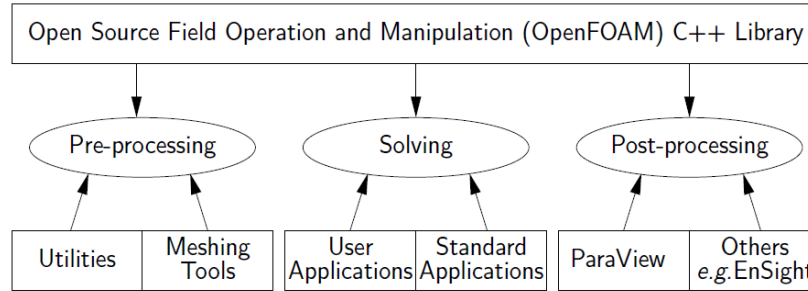
Figure 34: Overview of OpenFOAM® structure (source: https://OpenFOAM.org/ )
