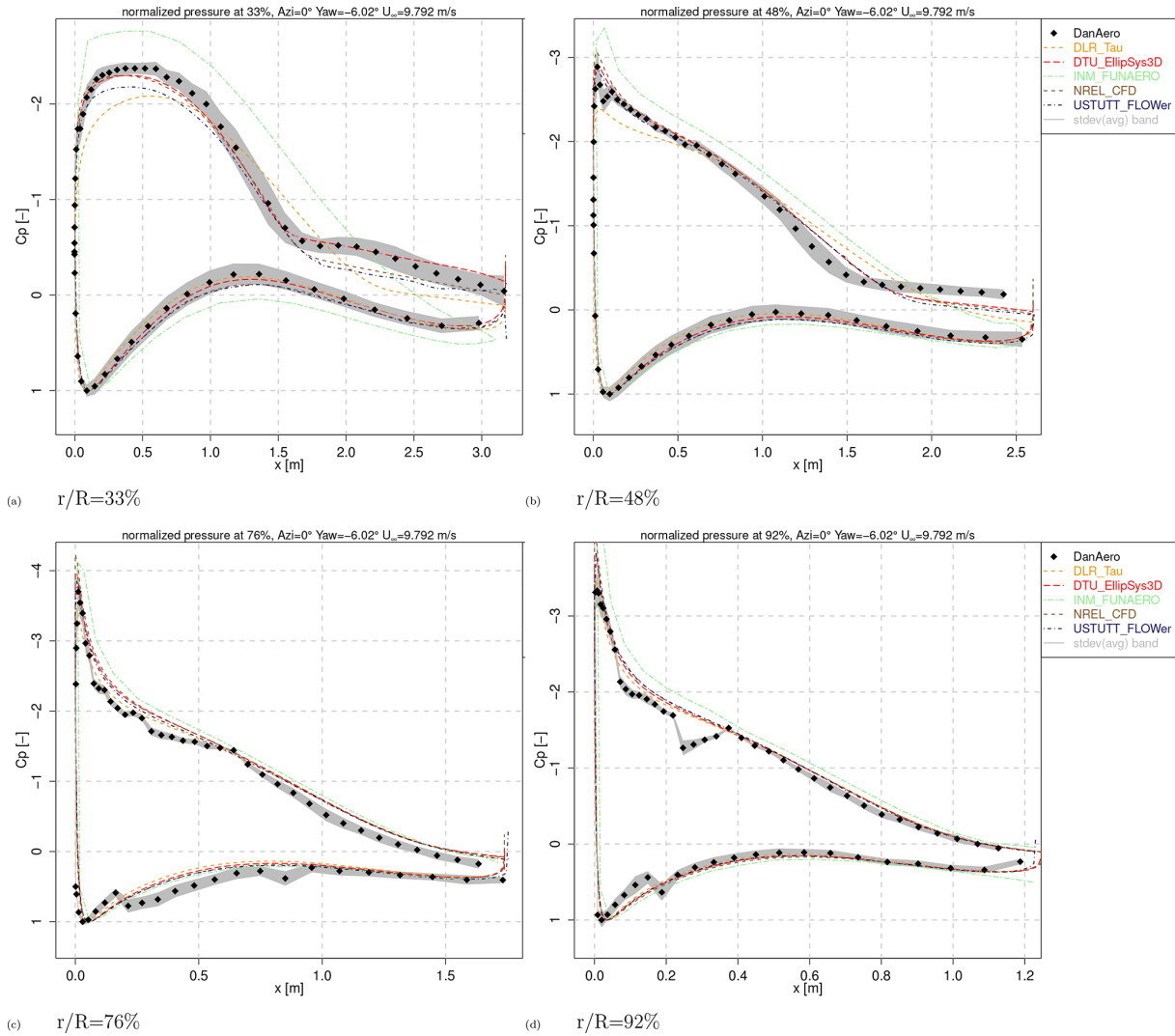
Figure 7. Pressure distribution comparison at 0° azimuth angle, Case IV.2.1. Animations of variation with an azimuth angle are available from the Supplement.
