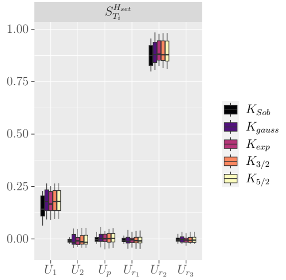
(b) \Gamma_{g_2}
