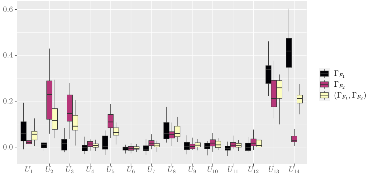
Figure 10 – Estimation of \hat{S}_i^{H_{set}} for the excursion sets \Gamma_{F_1} , \Gamma_{F_2} and the pair (\Gamma_{F_1}, \Gamma_{F_2}) with -q_1 = 420 N.m and q_2 = 7\% computed with the Sobolev input kernel and with n = 100 , m = 100 . 20 replicates.
