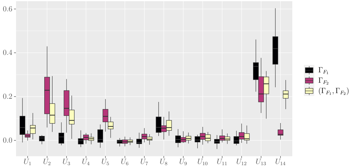
Figure 10 – Estimation of \hat{S}_i^{H-set} for the excursion sets \Gamma_{F_1} , \Gamma_{F_2} and the pair (\Gamma_{F_1}, \Gamma_{F_2}) with -q_1 = 420 N.m and q_2 = 7\% computed with the Sobolev input kernel and with n = 100 , m = 100 . 20 replicates.
