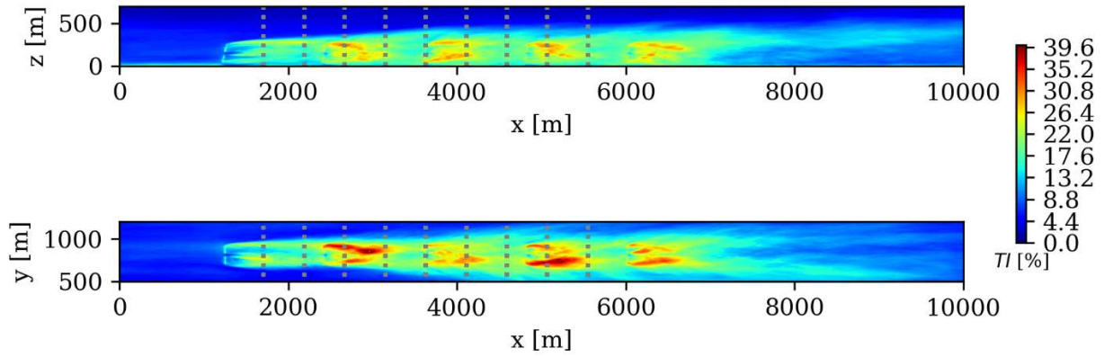
Figure 75. South Brittany vertical and horizontal cuts of mean TI at row position and hub height, respectively. Selected positions to extract vertical and horizontal profiles downstream of the first WT (dashed grey lines).
