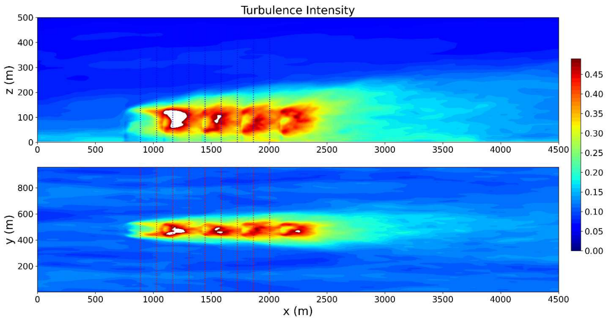
Figure 60 Vertical and horizontal cuts of turbulence intensity for crosswind case. Selected positions (from 1.5D to 13.5D) to extract vertical and horizontal profiles downstream of the first WT are shown by dashed lines.
