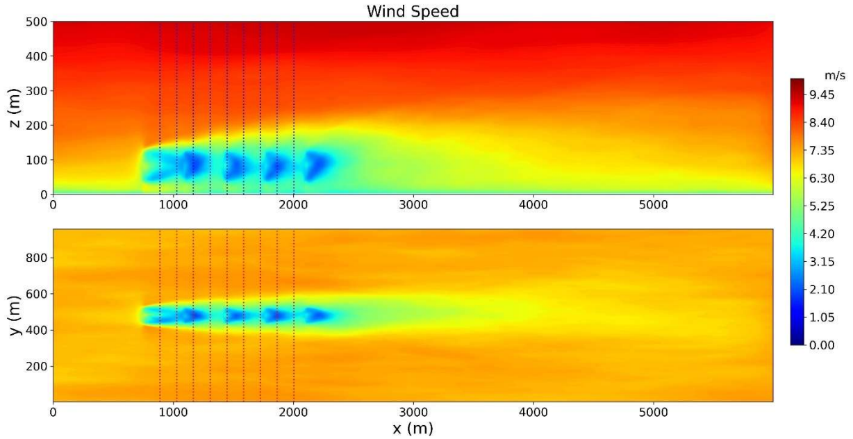
Figure 59 Vertical and horizontal cuts of mean wind speed for crosswind simulation. Selected positions (from 1.5D to 13.5D) to extract vertical and horizontal profiles downstream of the first WT are shown by dashed lines.
