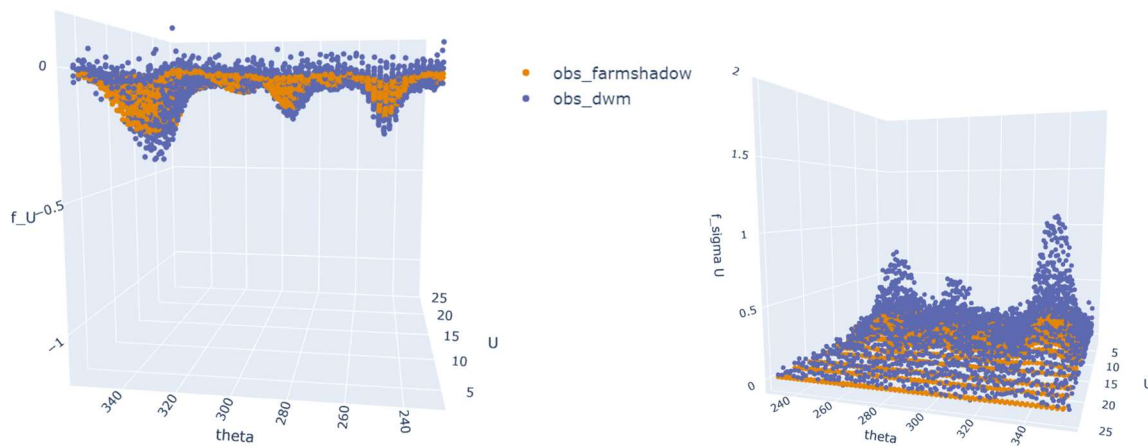
Figure 95: South Brittany: FarmShadow™ and DWM model results of the normalized f_u and f_{\sigma_u} .
