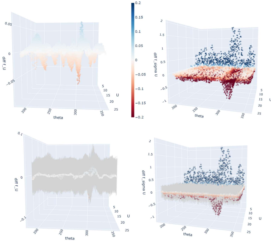
Figure 86 Teesside: Difference between GP predictions from FarmShadow™ and DWM coloured from red to blue (top). Error bars (grey) correspond to the std of the GP (bottom). Left: f_u . Right: f_{\sigma_u} .
