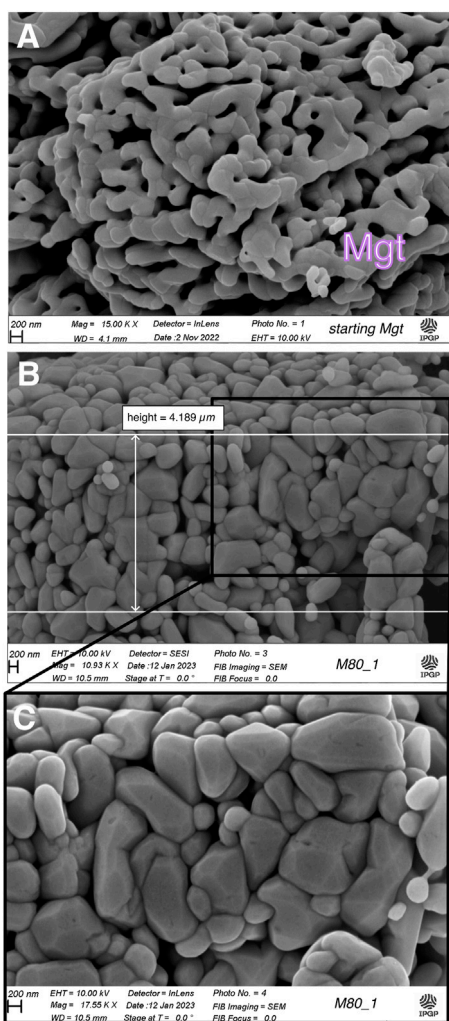
FIGURE 3 SEM images of (A) the starting magnetite compared to (B) magnetite after alteration at 80°C from M80_1 capsule. Note the higher mineral density and better crystallization after alteration. Mgt refers to magnetite. (C) Zoom of an altered magnetite surface from (B), highlighting mineral sharp edges.
