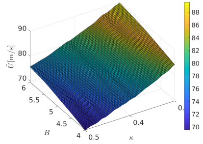
Figure 10: Response surface of \tilde{U}(r) for r = R/2
