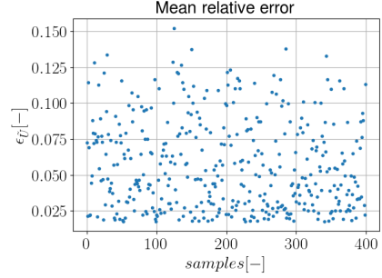
Figure 8: \varepsilon_{\tilde{U}} extracted from LES
