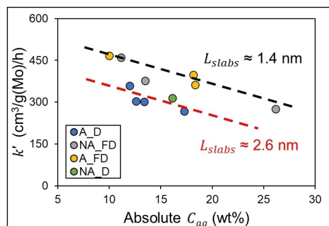
Figure 10. Evolution of the intrinsic catalytic performances evaluated by toluene hydrogenation with the amount of Mo involved in the slab aggregates ( Absolute C_{ag} )
