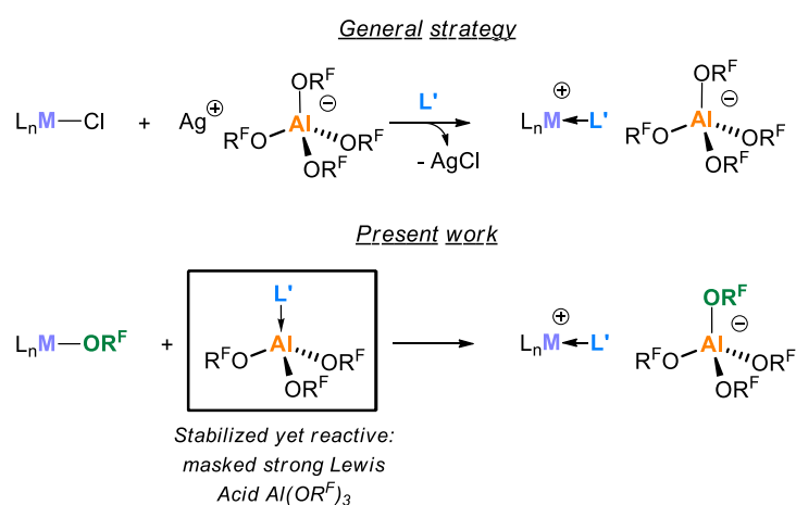
Scheme 1 – Comparative methods to access cationic complexes ( \text{R}^{\text{F}}=\text{C}(\text{CF}_3)_3 ).
